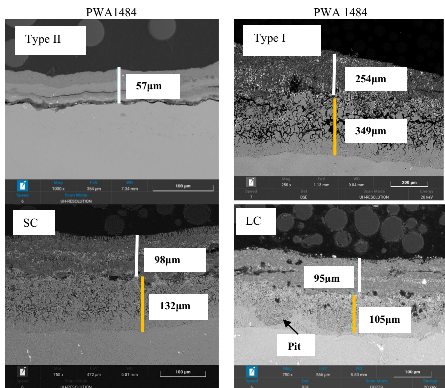
Fig. 6 Backscattered images of cross sections through alloy PWA 1484 samples covered with deposits ( 80\%\text{Na}_2\text{SO}_4 - 20\%\text{K}_2\text{SO}_4 ) exposed to air + 300 vppm \text{SO}_x gaseous atmosphere gas within SC test for 640 and LC test conditions for 560 h between 700–900 °C and isothermal Type I and Type II for 520 h at 900 and 700 °C, respectively
