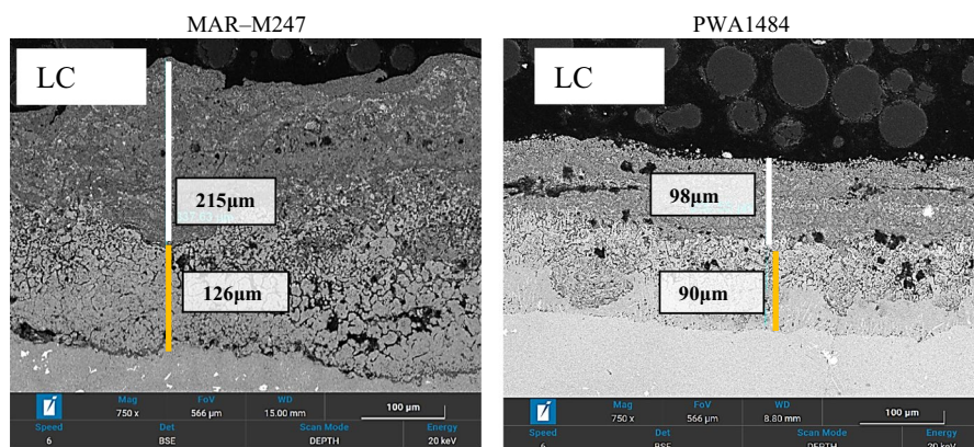
Fig. 3 Backscattered images of cross sections through alloy MAR-M247 and PWA 1484 samples covered with deposits ( 80\%\text{Na}_2\text{SO}_4 - 20\%\text{K}_2\text{SO}_4 ) exposed to air + 300 vppm SO x gaseous atmosphere gas within long cyclic test conditions for 560 h between 700–900 °C
