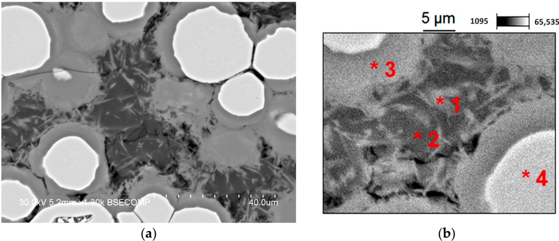
Figure 3. An area of the cross section of the composite obtained by SPS of Al-50 vol.% \text{Fe}_{66}\text{Cr}_{10}\text{Nb}_5\text{B}_9 (a). SPS conditions: temperature—570 °C, holding time—3 min, applied pressure—40 MPa. The points (1, 2, 3 and 4) in which the energy dispersive spectroscopy (EDS) analysis was conducted are marked in (b). BSE images.
