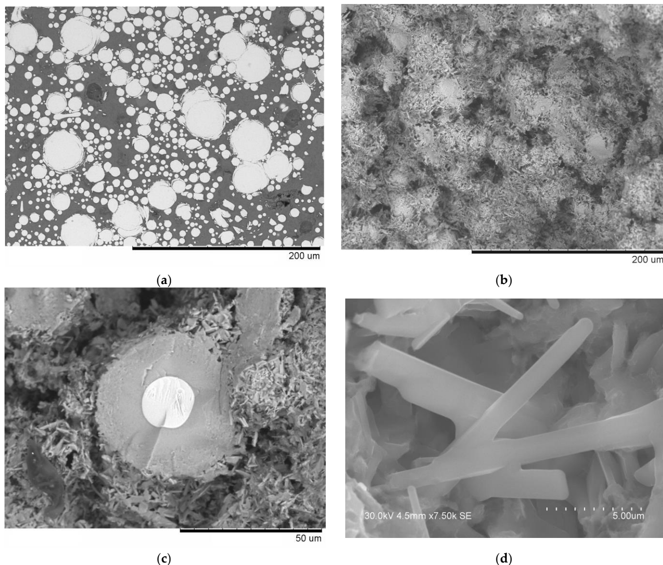
Figure 8. (a) Microstructure of the composite obtained by SPS of Al-20 vol.% Fe 66 Cr 10 Nb 5 B 9 Al powder. 3–10 \mu m. SPS conditions: temperature = 500 ^{\circ} C, holding time = 3 min, applied pressure = 40 MPa. (b) Fracture surface of the composite obtained by SPS and further annealed at 620 ^{\circ} C for 2 h. (c) An area of the fracture surface showing an unreacted Fe-based alloy core surrounded by platelets and needles of the intermetallic products. (d) The product of interaction with needle morphology. (a,b,c) BSE images. (d) Secondary electron (SE) image.
