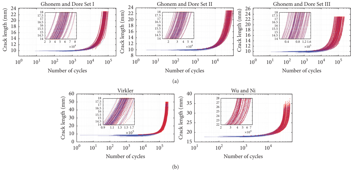
FIGURE 4: Comparison of raw (dots) and analytical (lines) crack length versus number of cycles for the 5 datasets.
