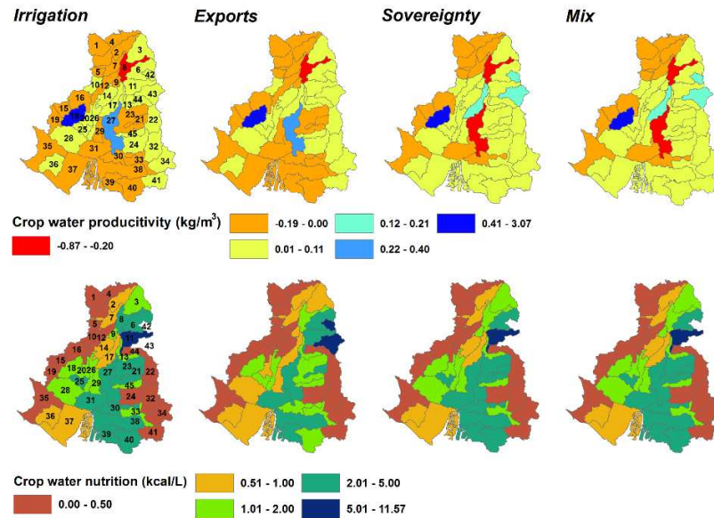
Fig. 9. Changes on median values for crop water productivity (kg/m 3 ) and crop water nutrition (kcal/L) between the proposed scenarios and baseline scenario.
