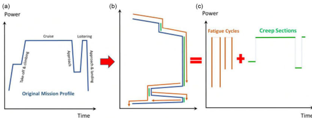
Figure 1. Schematic discretisation of mission profile using rainflow counting method (a) typical simplified flight mission; (b) water flows according to rainflow counting method; (c) equivalent discrete cycles and constant flight sections.
