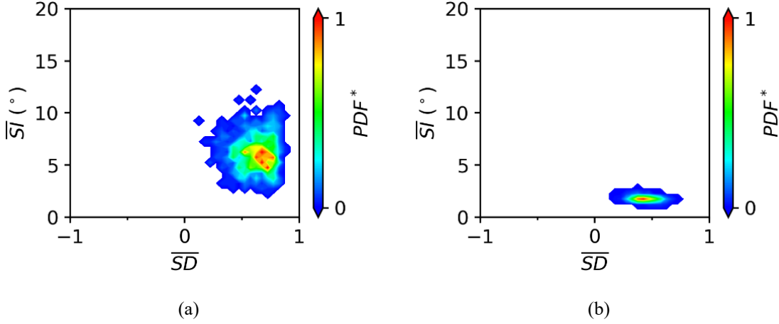
Fig. 10 Area-averaged SD-SI j-PDF maps for (a) Case 1 ( V_\infty=12.5 kts | 13.5 kRPM | MFCR=8.9 ) and (b) Case 2 ( V_\infty=12.5 kts | 26.5 kRPM | MFCR=17.5 ).
