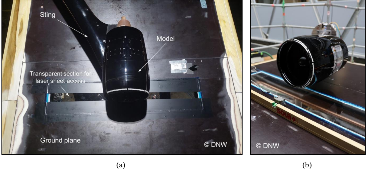
Fig. 3 Photographs of the model and ground plane: (a) Top view of the test article installed above the ground plane; (b) detail view showing the intake ground clearance.
