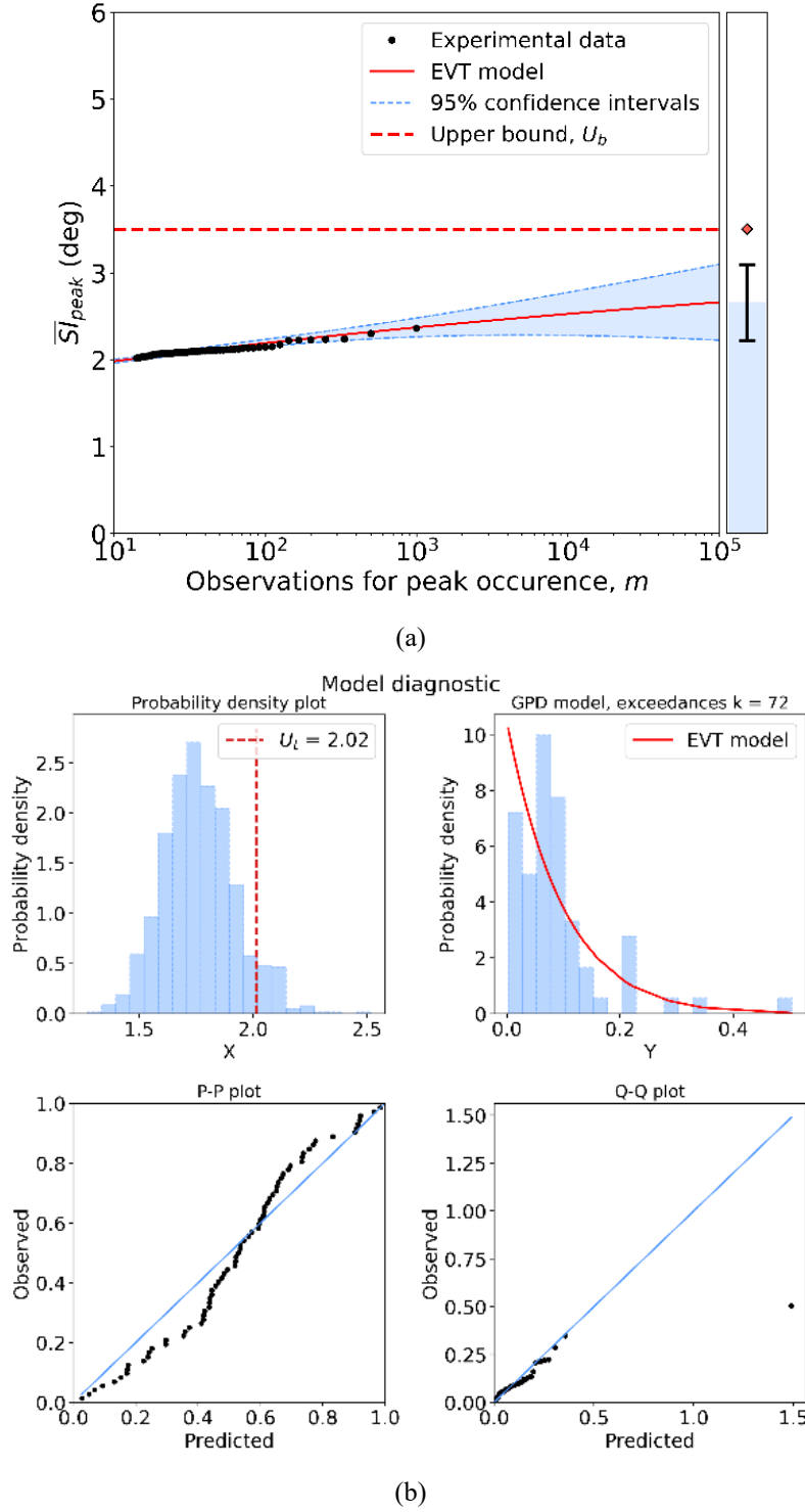
Fig. 13 (a) EVT return level plot of the peak area-averaged swirl intensity for Case 2 ( V_\infty=12.5 kts | 26.5 kRPM | MFCR=17.5). (b) Diagnostic plots for the EVT model.
