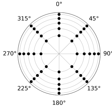
Fig. 5 8 \times 5 rake used for the assessment of swirl distortion at the AIP, following SAE guidelines [44].
