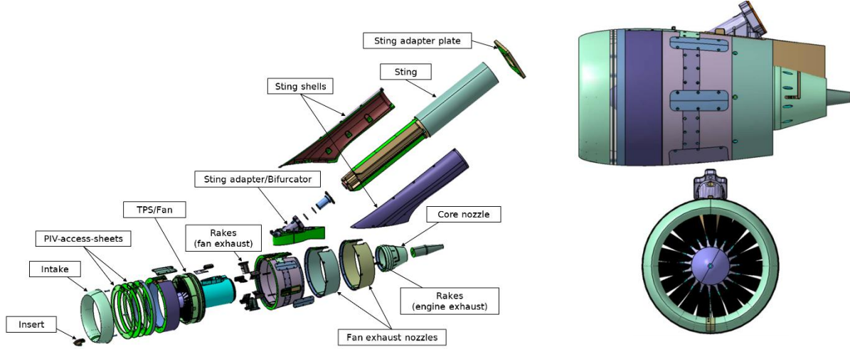
Fig. 2 Exploded and assembled views of the test article, illustrating the axisymmetric intake and the 10.2-inch TPS fan unit.
