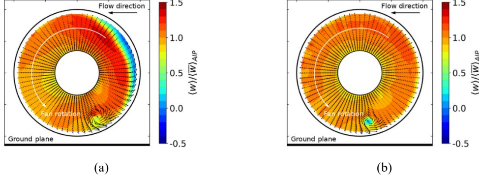
Fig. 7 Time-averaged, normalized out-of-plane velocity distributions at the Aerodynamic Interface Plane (AIP) for Case 1 (a) and Case 2 (b).
