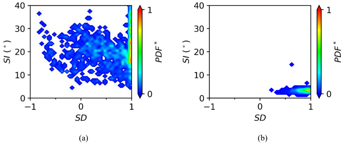
Fig. 11 SD – SI j-PDF maps for (a) Case 1 ( V_\infty=12.5 kts | 13.5 kRPM | MFCR=8.9 ) and (b) Case 2 ( V_\infty=12.5 kts | 26.5 kRPM | MFCR=17.5 ) evaluated at r/R_{AIP} = 0.956 .
