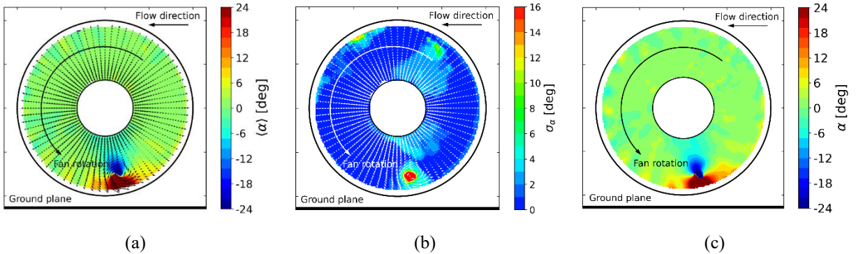
Fig. 9 Time-averaged (a), standard deviation (b), and instantaneous (c) swirl angle distributions at the Aerodynamic Interface Plane (AIP) for Case 2 ( V_\infty=12.5 kts | 26.5 kRPM | MFCR=17.5 ).
