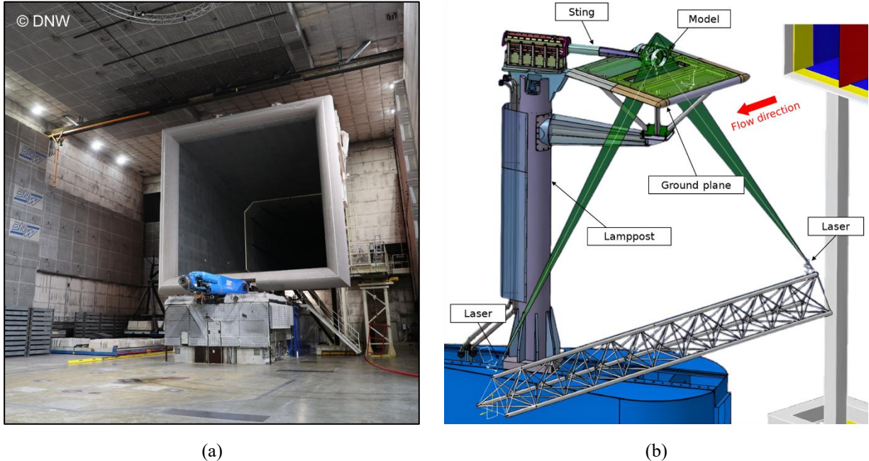
Fig. 1 DNW-LLF experimental facility: (a) Photograph of the empty wind tunnel in open test-section configuration; (b) schematic of the test set-up.
