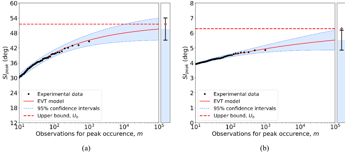
Fig. 14 EVT return level plots of the peak swirl intensity evaluated at r/R_{AIP} = 0.956 . for (a) Case 1 ( V_\infty=12.5 kts | 13.5 kRPM | MFCR=8.9) and (b) Case 2 ( V_\infty=12.5 kts | 26.5 kRPM | MFCR=17.5).
