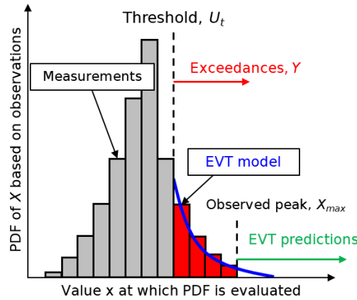
Fig. 6 Extreme Value Theory (EVT) framework showing the Peak-Over-Threshold (POT) approach.
