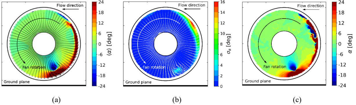
Fig. 8 Time-averaged (a), standard deviation (b), and instantaneous (c) swirl angle distributions at the Aerodynamic Interface Plane (AIP) for Case 1 ( V_\infty=12.5 kts | 13.5 kRPM | MFCR=8.9 ).
