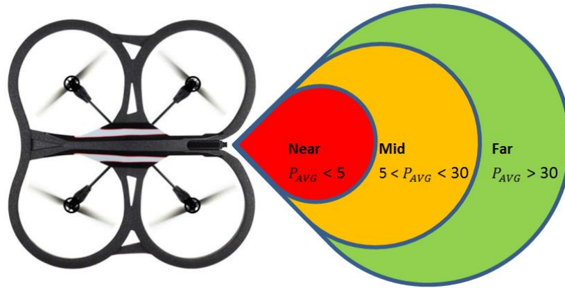
Figure 5. Relationship between flocking zones and detected pixel values.
