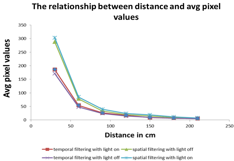
Figure 8. The effects of spatial and temporal vision filtering under different lighting conditions. The spatial filtering technique has a higher number of average pixels value P_{AVG} than the temporal filtering technique at closer distances but similar values at larger distances. For both approaches, the maximum visual distance Visual_{max} is about 200 cm.
