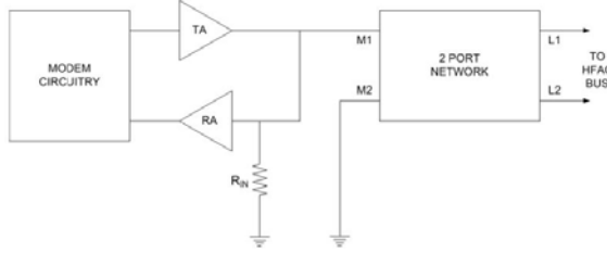
Fig. 4. Simplified representation of the modem line interface stage for a voltage-fed system.
