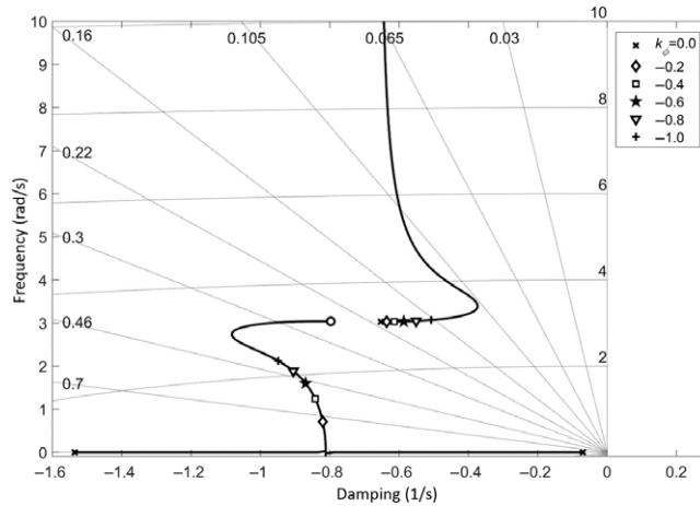
Figure 21. Eigenvalue loci for FXV-15 lateral-directional dynamics with varying k_\phi ; k_1 = 0 .
