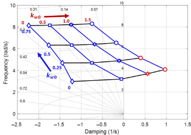
Figure 20. Short-period pitch-heave mode eigenvalue loci map for varying feedback of vertical velocity and acceleration to X_b ; FXV-15 in A-model, 135kts, \gamma = 3.5^\circ .
