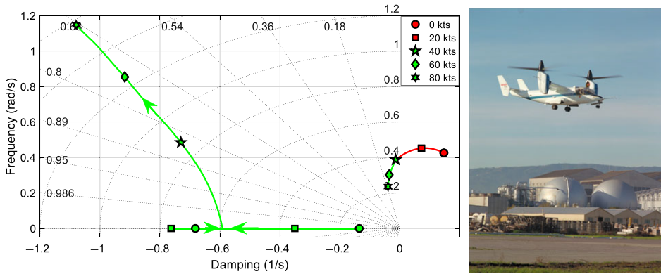
Figure 4. Longitudinal eigenvalues as a function of speed for the FXV-15 in H-mode; descent \gamma = 3.5^\circ XV-15 in hover (photo NASA).
