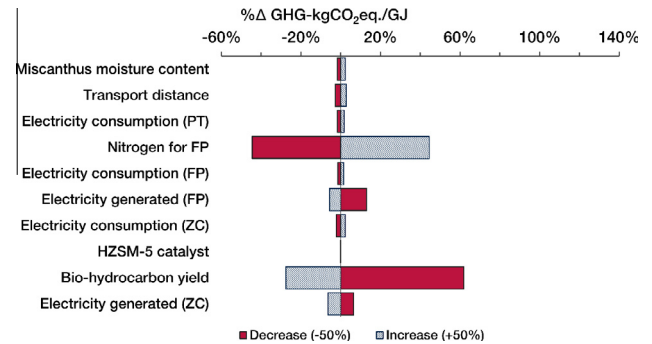
Fig. 12a. Sensitivity of GHG emissions (kg CO 2 eq./GJ) from the zeolite cracking pathway to \pm 50\% variation in parameters (PT, FP and ZC denote pretreatment, fast pyrolysis and zeolite cracking, respectively).
