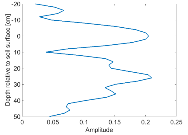
Figure 5: The depth profile produced from an FFT of the phase history at the pixel corresponding to the position of the buried trihedral (ie using the SMC-linearized phase shown in Figure 4).
