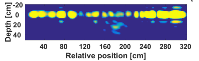
Figure 6: The final VB-SAR image along the 3m transect derived from the low resolution DInSAR stack.
