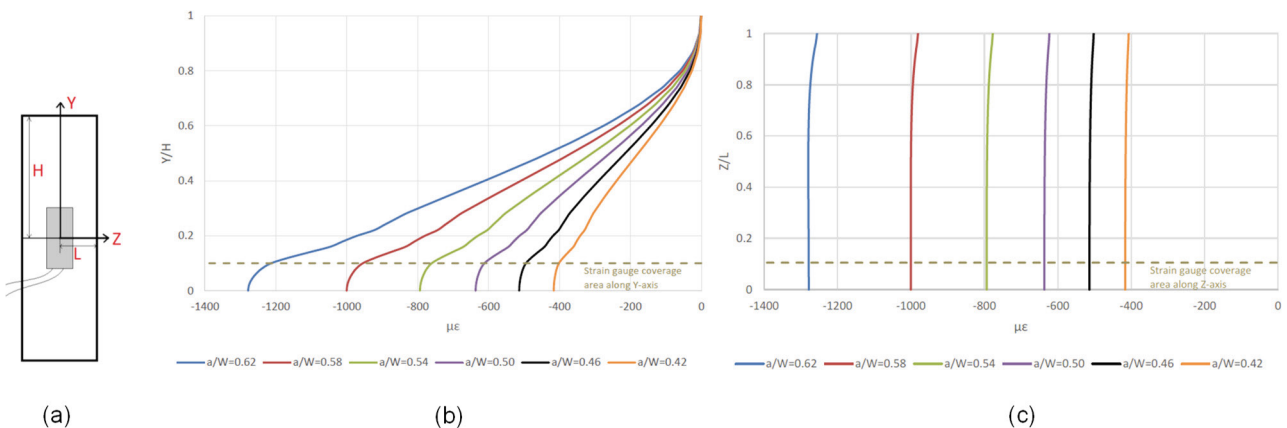
Figure 3: (a) BFS measurement area in the experiment and FE simulation (b) an example of strain variation along Y-axis at different crack lengths (c) strain variation along Z-axis at different crack lengths
