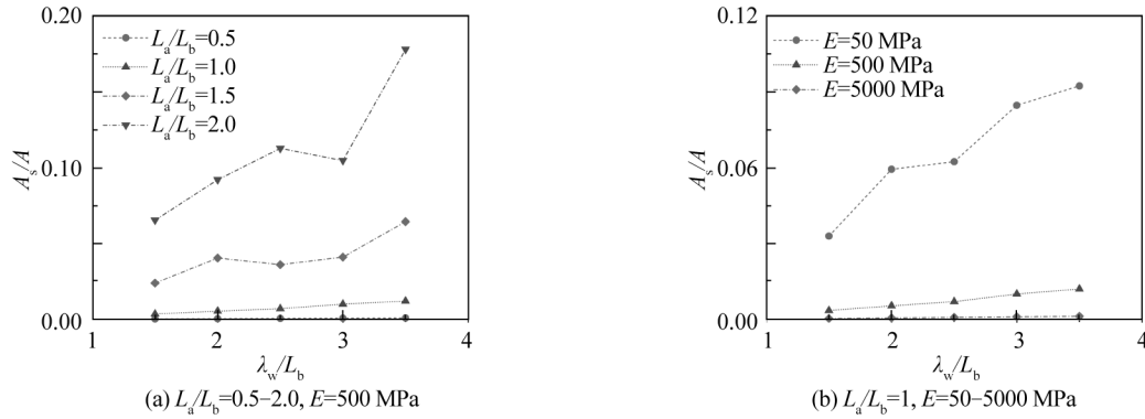
Fig. 17. Displacement amplitude measured at the free edge of the flexible tail in the steady stage with: (a) L_a/L_b = 0.5-2.0 and E = 500 MPa; (b) L_a/L_b = 1 and E = 50-5000 MPa.
