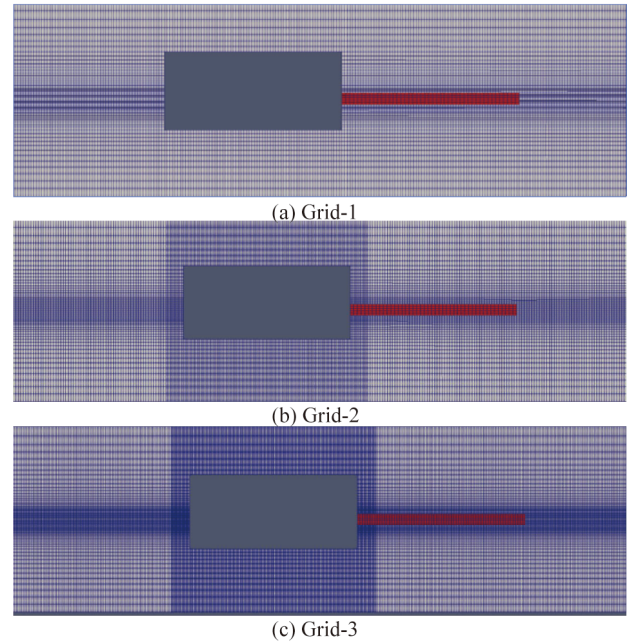
Fig. 4. Local grid refinement of (a) Grid-1, (b) Grid-2 and (c) Grid-3, in which computational solid mechanics (CSM) grids are in red.
