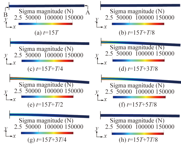
Fig. 15. Deformation and stress distribution of the wave attenuator, with L_a/L_b = 2 , E = 500 MPa, and \lambda_w/L_b = 3.5 .
