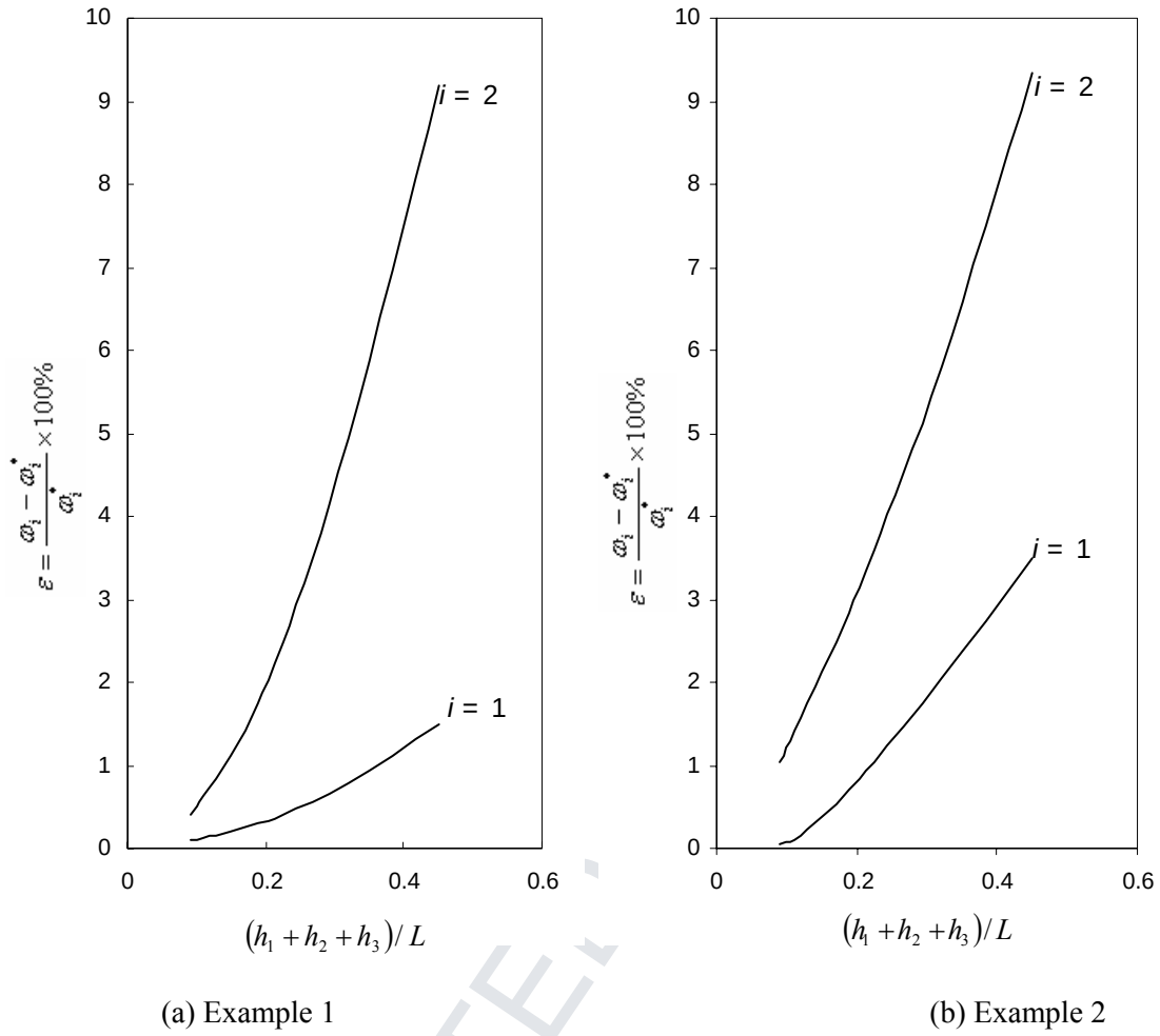
Fig.5. Effect of thickness to length ratio on the natural frequencies of examples 1 and 2.
