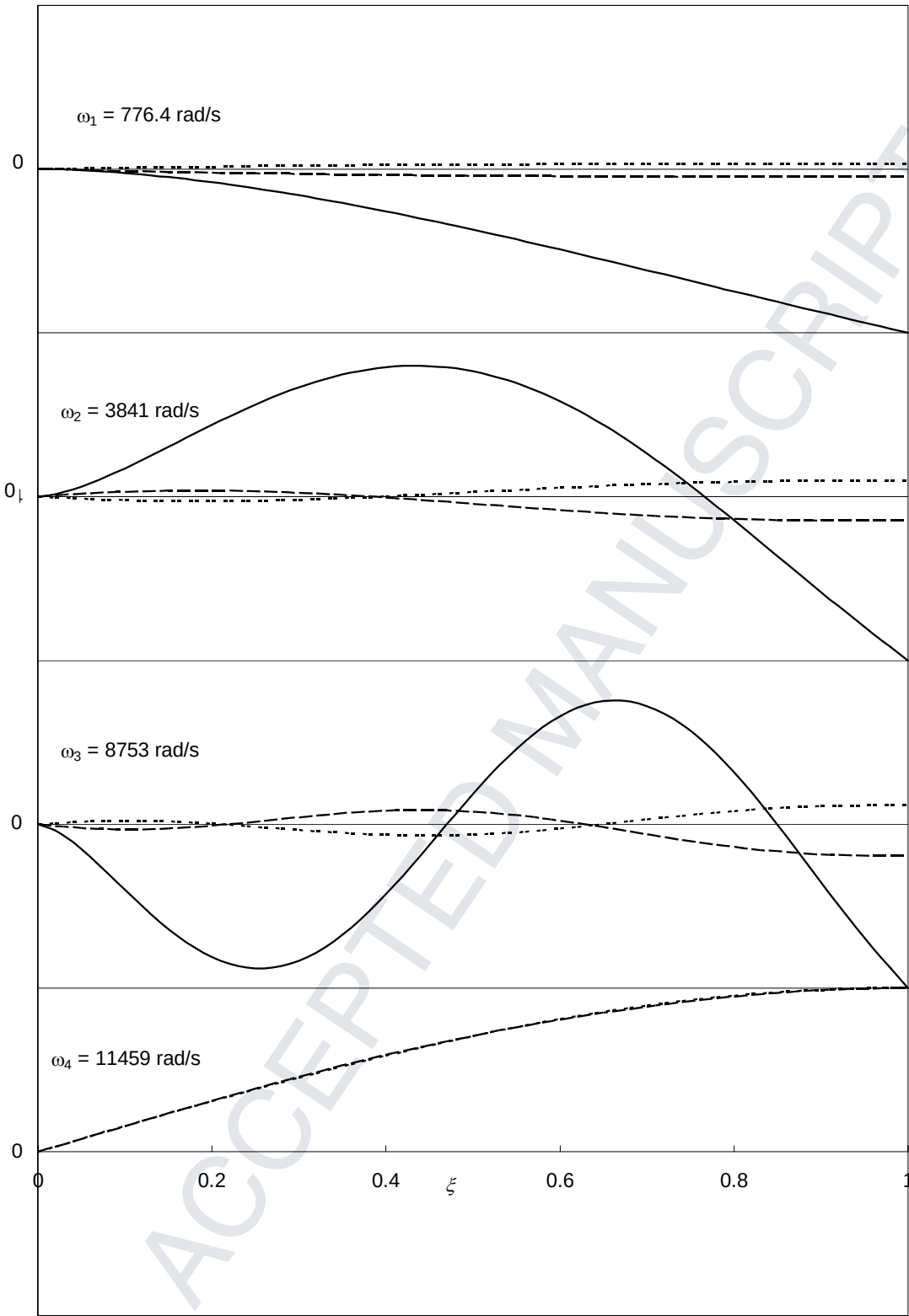
Fig. 4. Natural frequencies and mode shapes of the three-layered sandwich beam of example 2. — W ; - - - U_1 ; ···· U_3
