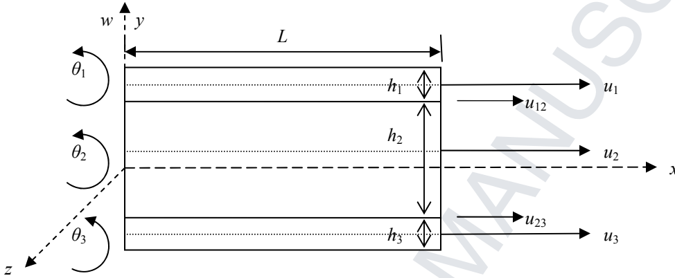
Fig. 1. The coordinate system and notation for a three-layered sandwich beam
