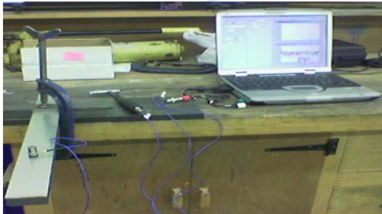
Fig. 6 Experimental set up for modal testing of a cantilever sandwich beam.
