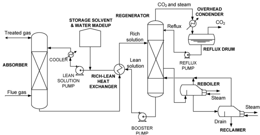
Figure 4.4 Typical configuration of solvent-based adsorption CO 2 capture process (Thitakamol, B., Veawab, A., Aroonwilas, A, 2007)
