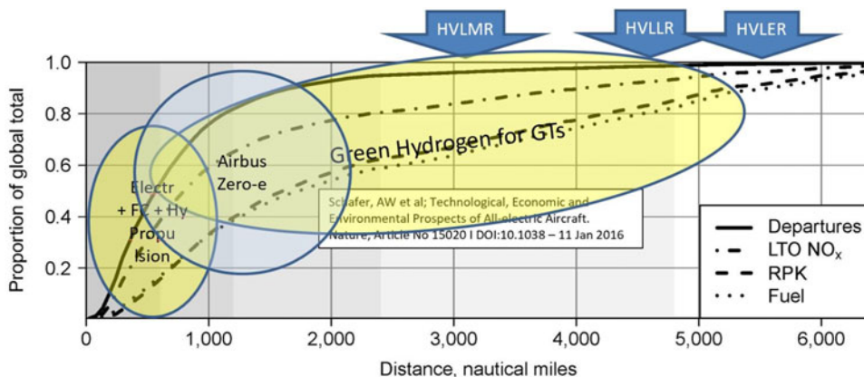
Figure 7. HVLMR, HVLLR and HVLER capabilities (8) annotated by the authors and including the authors understanding of the Airbus Zero-e concepts (23) .
