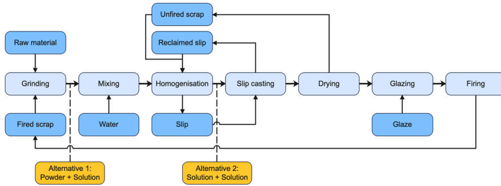
Figure 1 Manufacturing process of SCs as well as the potential graphene inclusion points
