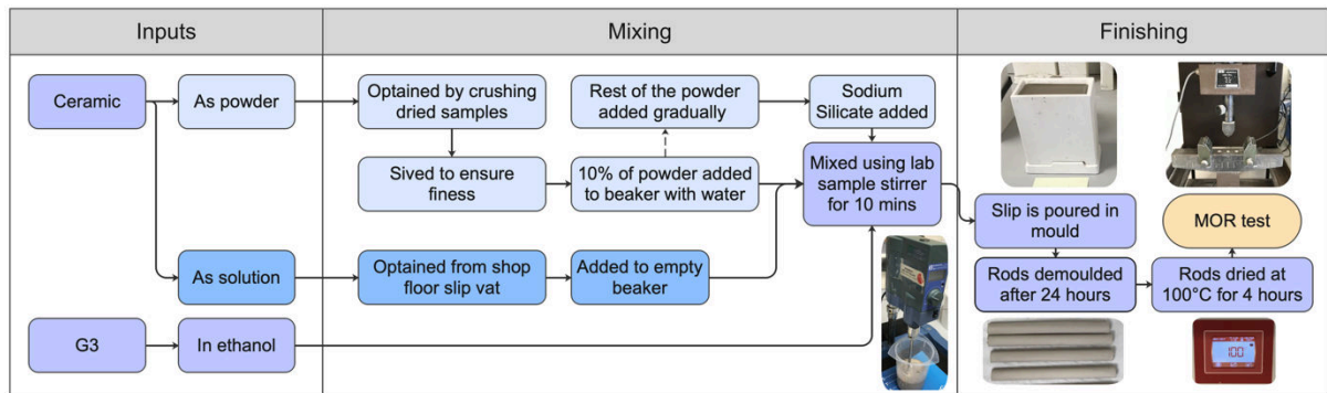
Figure 2 Slip casting process
