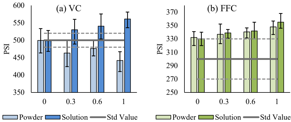
Figure 5 MOR results along with standard strength values for a) VC and b) FFC
