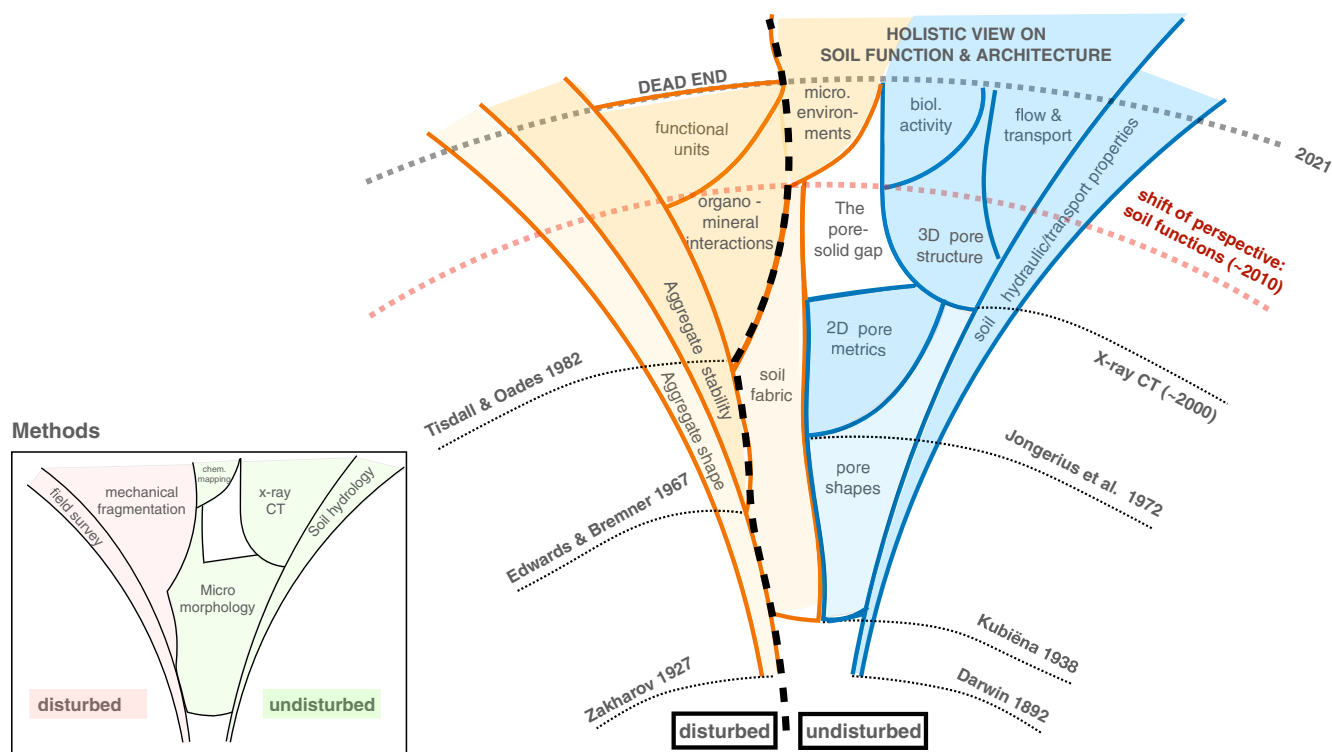
FIGURE 1 Historical development of exploring soil structure. The pore perspective is in blue, the solid perspective in ochre. Dark colours and light colours indicate quantitative and qualitative analysis, respectively. New branches of developments with respect to research foci are marked by milestone publications or new technical developments
