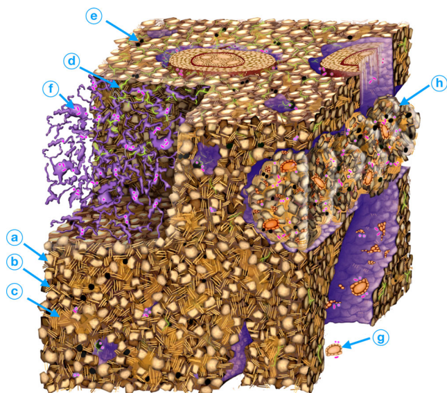
FIGURE 2 Schematic sketch of the typical structural organization of fine-textured soil. The organo-mineral soil matrix is composed of quartz grains (a), clay minerals (b), organic coatings on mineral surfaces (c), amorphous, particulate organic matter (e) and organic tissues (g). In the upper left corner, the highly connected pore space between mineral grains is illustrated, where fungi (d) frequently associated with roots and bacteria (f) are active. As an example of biotic mixing, an earthworm cast (h) is drawn on the right side. The hotspots of biological activity are locations where carbon sources are available for the microbiome, living in pores of appropriate size. Mobile organic and mineral compounds may diffuse through the connected pore space within the rigid skeleton of mineral grains, leading to a heterogeneous organo-mineral soil matrix. The drawing is not meant to be true to scale to better illustrate the relevant components (Graphics: Lisa Vogel, www.lisavogel-illustration.de )
