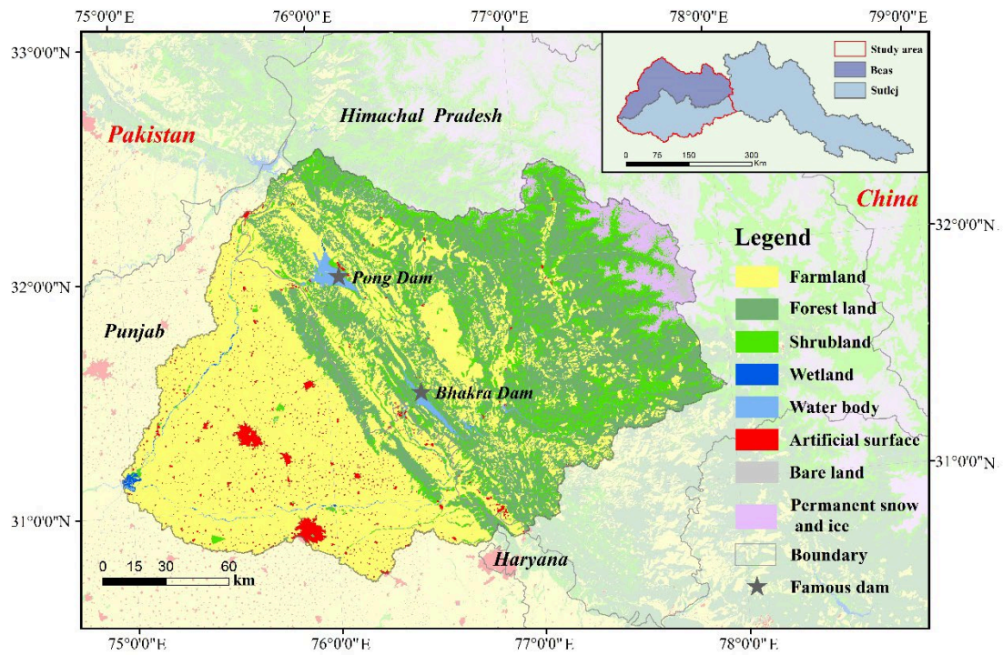
Fig. 1. Geographical location and land cover of the study area.
