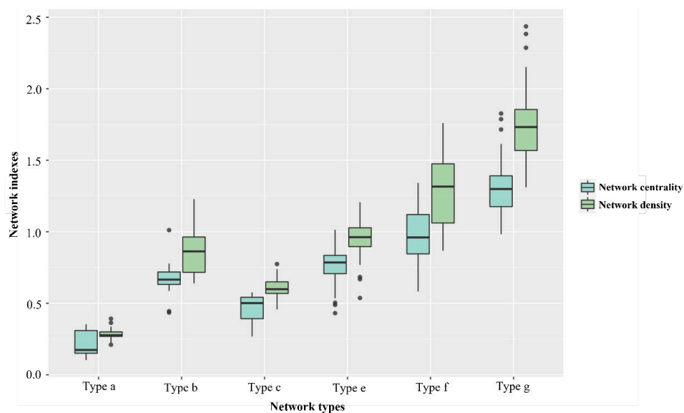
Fig. 8. Boxplot of network indexes for different water-related ES network types
