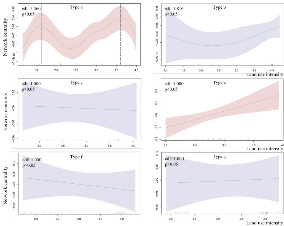
Fig. 9. Correlations between network centrality and land use intensity across various
