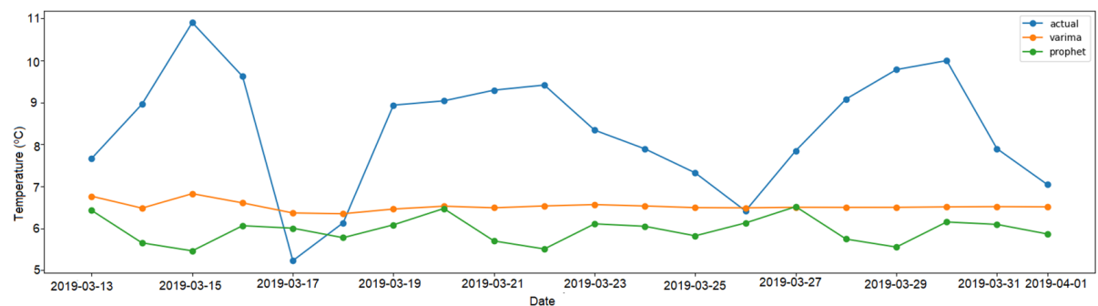
Figure 7. Comparison of VARIMA and FB Prophet forecasts with actual temperature value.
