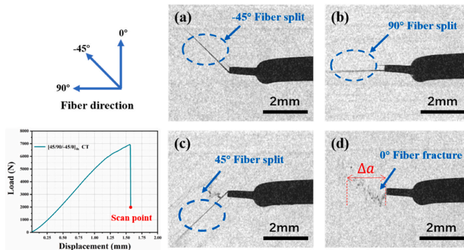
Fig. 2. Typical CT images of damage in (a) -45° ply, (b) 90° ply, (c) 45° ply, (d) 0° ply of [45/90/-45/0]_{4s} specimen at HTW. Note. These images were captured immediately after the peak load, and \Delta a is the 0° crack increment.
