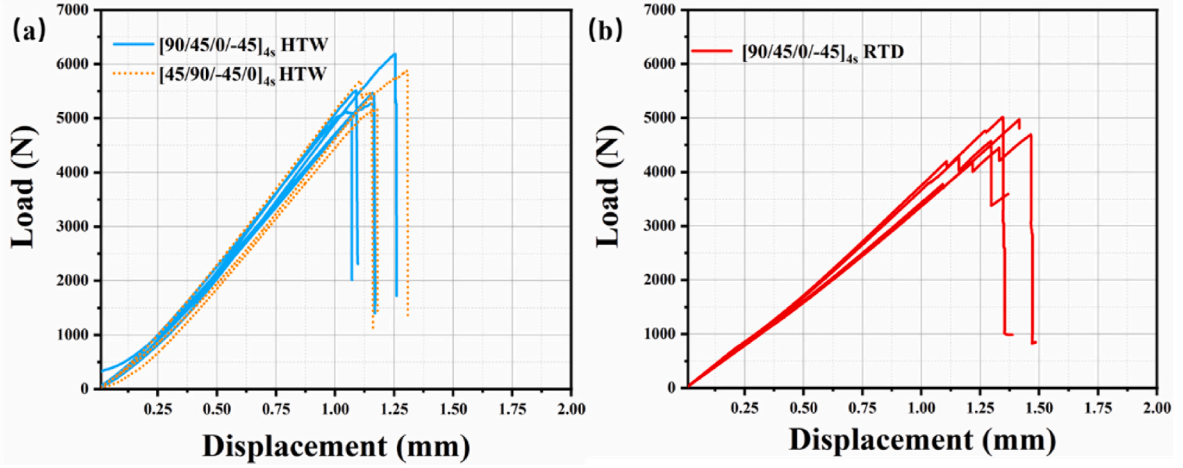
Fig. 3. (a) Load-displacement curves of two sets of specimens at HTW. Note. The peak load of [90/45/0/-45]_{4s} and [45/90/-45/0]_{4s} are 5514 \text{ N} \pm 407.3 and 5587 \text{ N} \pm 369.3 , respectively. (b) Load-displacement curves of specimens at RTD. Note. The peak load is 4812 \text{ N} \pm 216.3 .
