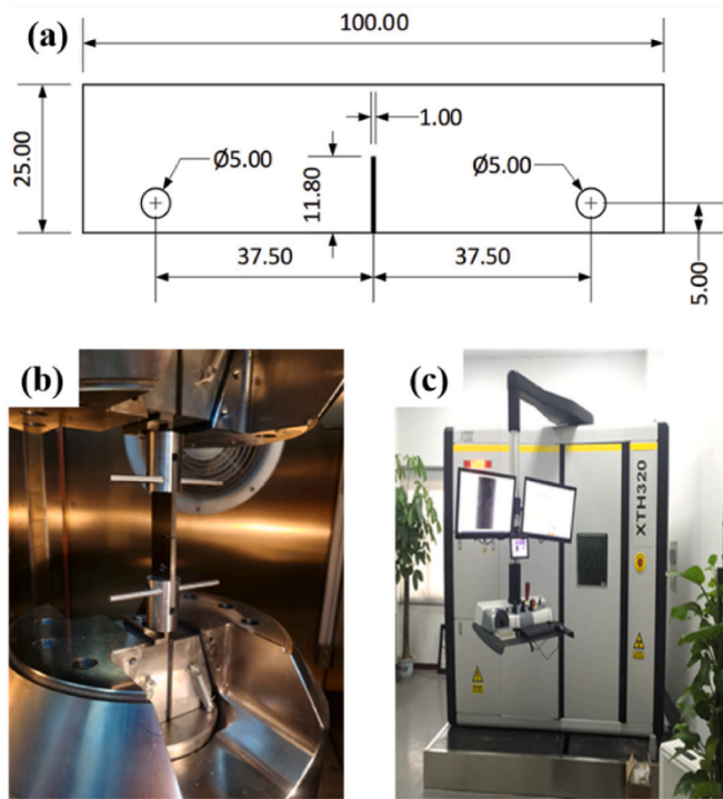
Fig. 1. Specimen and test set-up (a) geometry and dimensions of specimen, based on ASTM E1922; (b) test jig in chamber; (c) CT scanner, NIKON XTH 320 LC CT.
