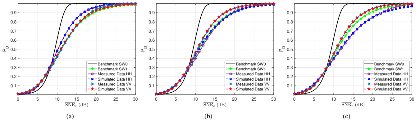
Fig. 3 P_D versus \overline{\text{SNR}}_c for HH and VV polarization curves using measured and simulated drones data: (a) Venom VN10 at 9.1 GHz, (b) Parrot AR.DRONE at 14 GHz, (c) AscTec Pelican at 9.2 GHz.
