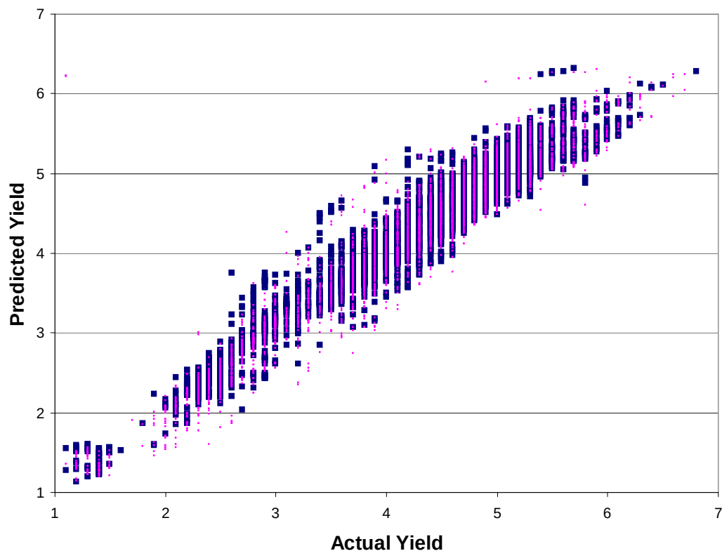
Figure 3 Performance of neural network for winter wheat yield (t/ha) – the yield predicted by the neural network is plotted against the actual yield from the full model which the neural network seeks to emulate.
