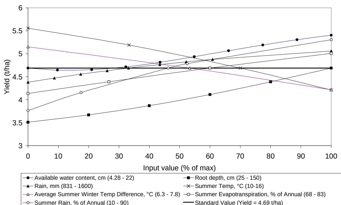
Figure 10 Testing the responses of the neural network predicting the winter wheat yield. Each line shows the effect on the output (yield) of changing a single input value over the specified range.
