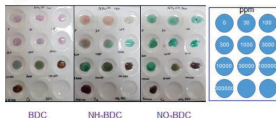
Fig. 3. Co based MOF responses to aqueous ammonia (0 – 300,000 ppm)
