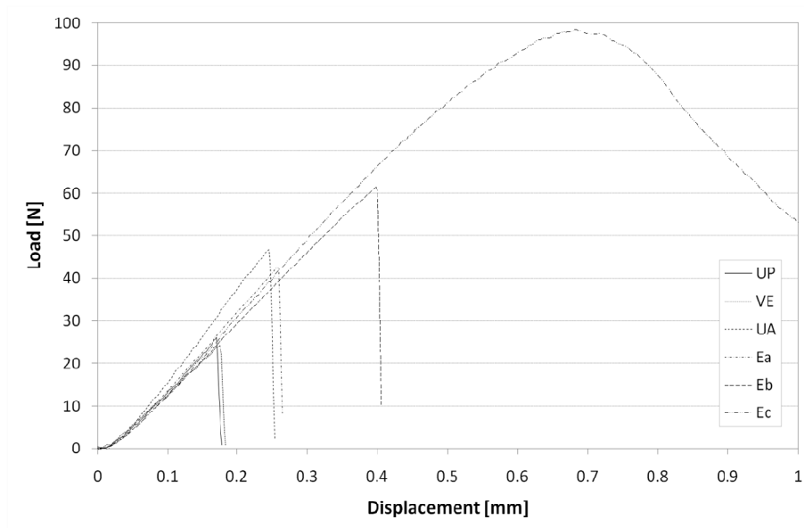
Figure 1: Representative load/displacement curves obtained by testing notched specimens of cast resin in three-point bending configuration for toughness measurement
