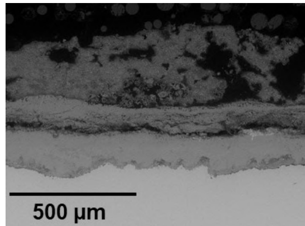
a) b) Fig. 4. Back-scattered electron images of T91 exposed in simulated oxy-fired combustion gases at 600 °C for 1000 h; a) without any deposit (D0), b) with the deposit with high levels of SO 4 (D1).
