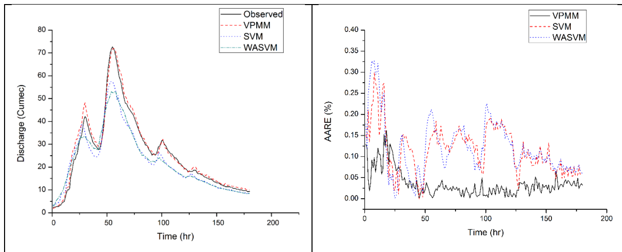
Fig. 7 Routed hydrograph and AARE for flood event 3 using VPMM, SVM and WASVM.
