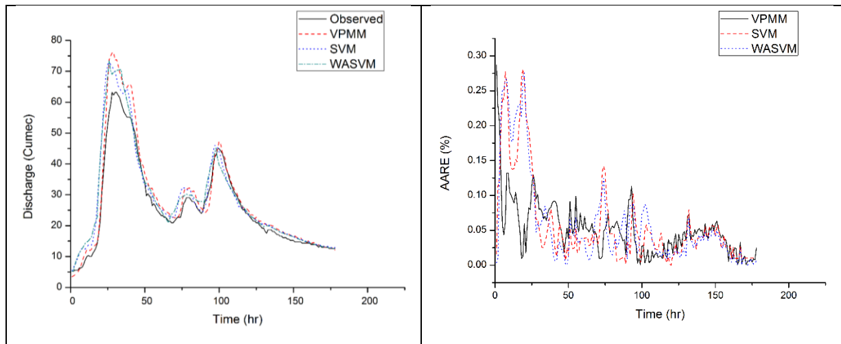
Fig. 6 Routed hydrograph and AARE for flood event 2 using VPMM, SVM and WASVM.
