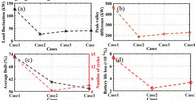
Fig. 7. Quantitative performance comparison of different methods on GEVs fleet. (a) load fluctuation mitigation; (b) peak-shaving difference; (c) battery cycles and DoD; (d) quantified battery life loss.
