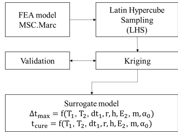
Fig. 2. Surrogate model construction methodology.
