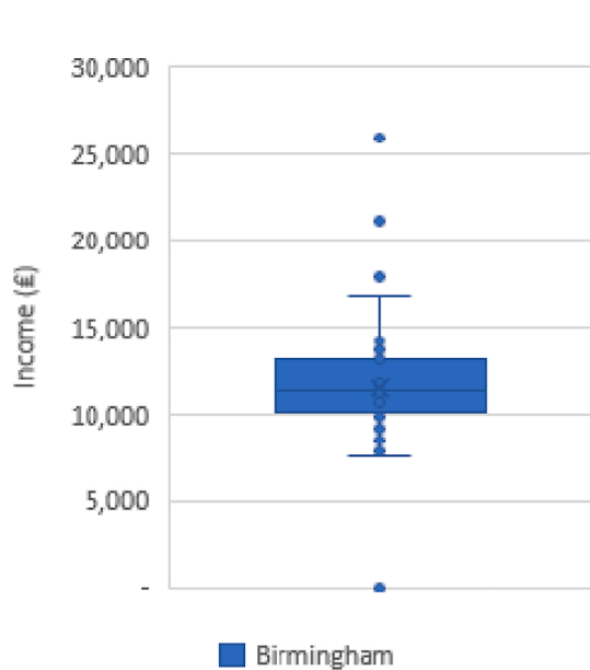
Fig. A1. Boxplot of the PC's income in Birmingham.
