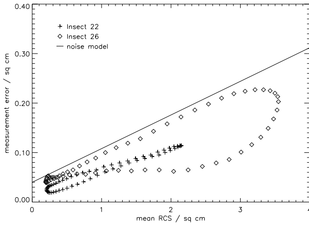
Figure 2: Measurement noise standard deviation as a function of mean RCS for the insects of [10].
