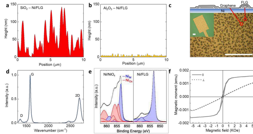
Fig. 1. AFM line scan of sputtered Ni films after graphene growth using a Si-SiO 2 substrate without (a) and with (b) an \text{Al}_2\text{O}_3 adhesion layer. (c) Optical micrograph of a graphene-passivated Ni electrode, including a cartoon indicating areas with different numbers of graphene layers. Scale bars are 50 \mu\text{m} . (d) Raman spectrum of few-layer graphene on Ni. (e) XPS of Ni 2p 3/2 region of sputtered Ni (Ni/NiO x – black) and Ni after multilayer graphene growth (Ni/FLG – green), with peak fitting indicating metallic nickel (Ni M ) and nickel oxide (NiO x ). (f) Magnetic moment measured at room temperature by DC-mode SQUID magnetometry of graphene-passivated Ni films for magnetic fields parallel (grey, solid) and perpendicular (black, dots) to the plane of the film.
