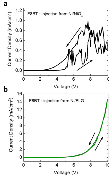
Fig. 3. Current density hysteresis as a function of voltage for hole injection into F8BT using (a) unprotected sputtered Ni electrodes and (b) graphene-passivated Ni. The arrows indicate the direction of voltage sweep.
