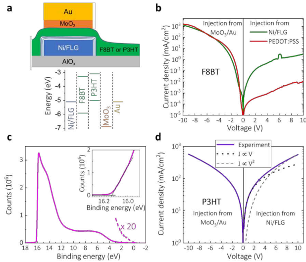
Fig. 2. (a) Schematic representation of the device structure used. (b) Comparison of hole injection into F8BT from graphene-passivated Ni (green) and PEDOT:PSS (red) bottom contacts, each using a top contact of MoO 3 / Au. (c) Binding energy, referenced to the Fermi level, measured on a Ni/FLG sample by means of UPS (excitation light with energy h\nu = 21.21 eV). The inset shows the high binding energy part of the spectrum used to extract the cut-off energy E_{co} . The work function \phi is calculated as \phi = h\nu - E_{co} . For better visualization, the part of the curve at the Fermi level is also shown after 20-fold magnification (dashed line). (d) Hole injection into P3HT from graphene-passivated Ni, with MoO 3 /Au top contact.
