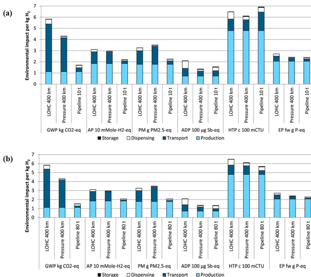
Fig. 13. Environmental impacts of different cases considered (a) Hydrogen demand at 10 t/d and transportation distance of 400 km (b) Hydrogen demand at 80 t/d and transportation distance of 400 km. [236].
