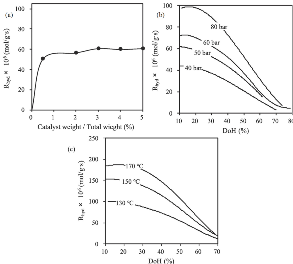
Fig. 5. Hydrogenation rate of dibenzyltoluene over a Ru/Al 2 O 3 catalyst at varying (a) catalyst weights (130 °C, 50 bar), (b) pressures and DoH (130 °C), and (c) temperatures and DoH (80 bar) [65].
