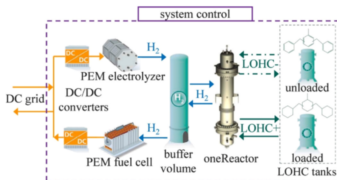
Fig. 9. Process flow diagram of a one-reactor concept for LOHC energy storage system integrated with PEM fuel cell and electrolyzer [182]. LOHC = liquid organic hydrogen carrier; PEM = proton exchange membrane.
