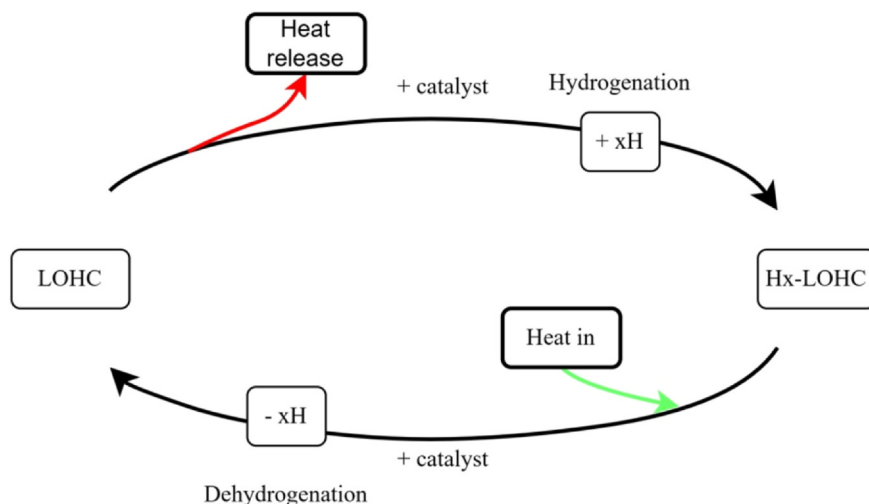
Fig. 3. Hydrogenation-dehydrogenation reaction steps in LOHCs technology. LOHCs = liquid organic hydrogen carriers.
