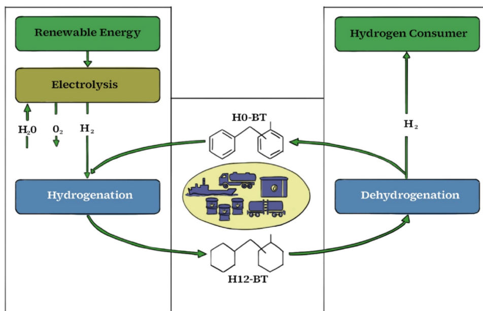
Fig. 2. Schematic representation of the LOHC cycle for renewable energy storage and distribution. LOHC = liquid organic hydrogen carrier.
