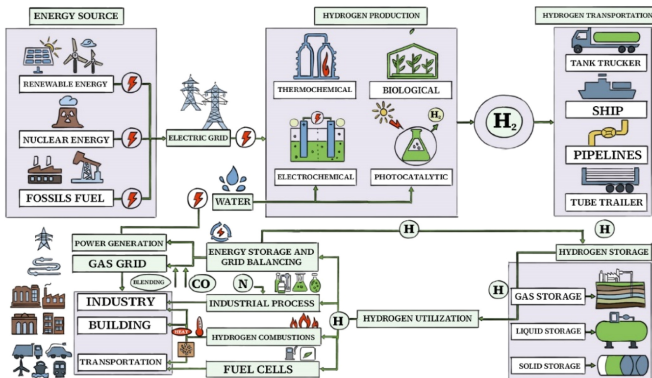
Fig. 11. A synopsis of technologies for HPTSU [198]. HPTSU = hydrogen production, transportation, storage, and usage.
