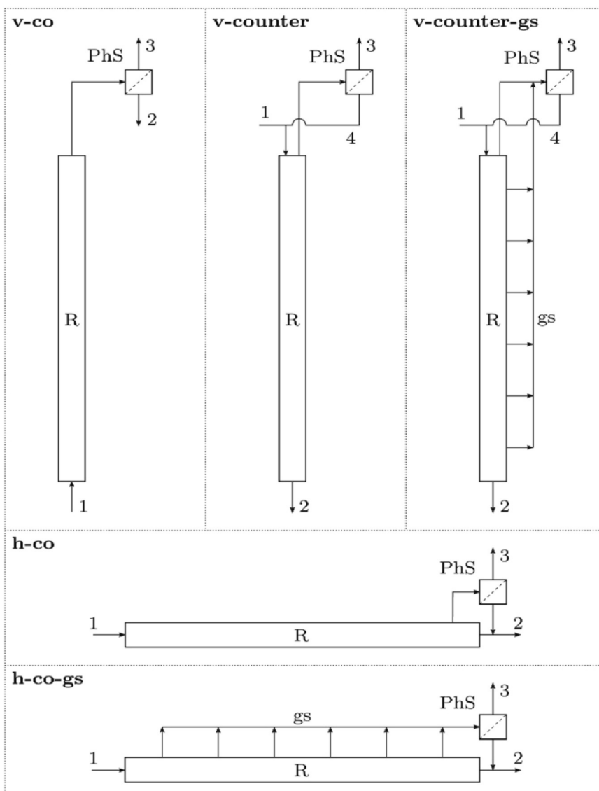
Fig. 8. Different fixed bed arrangement studied by Heublein et al. [175]. v-counter and v-co represents counter-flow and co-flow, respectively, with the liquid feed (1) entering the reactor at the bottom and both the liquid product (2) and the purified hydrogen gas (3) leaving the reactor at the top.
