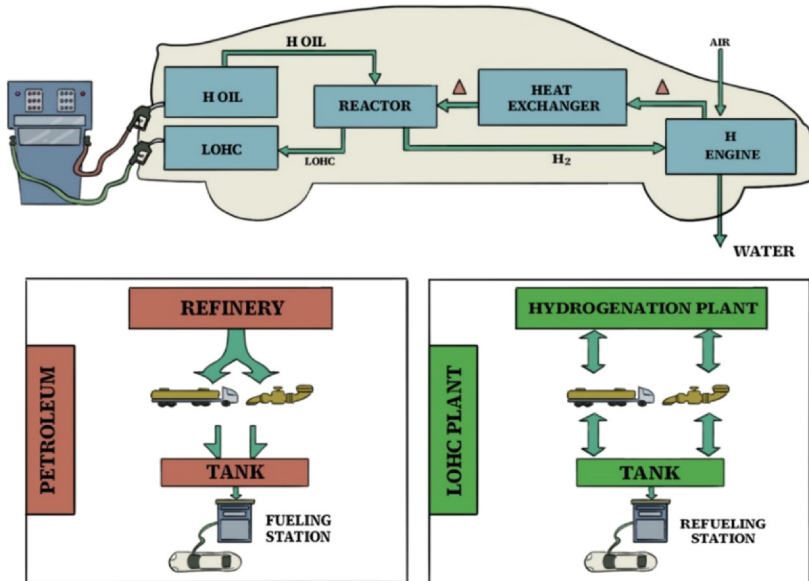
Fig. 12. Prototype of H 2 automobile using LOHC for H 2 supply. LOHC = liquid organic hydrogen carrier.
