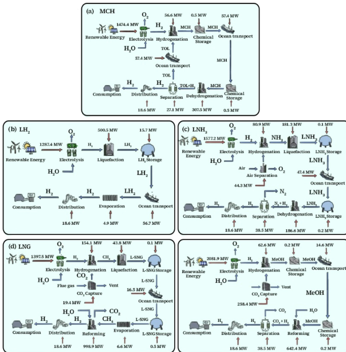
Fig. 14. Energy demand in various hydrogen carriers [245,246].
