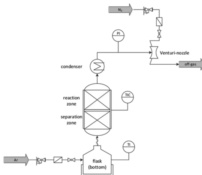
Fig. 10. Reactive distillation reactor set-up used for the dehydrogenation of H12-BT. [180].
