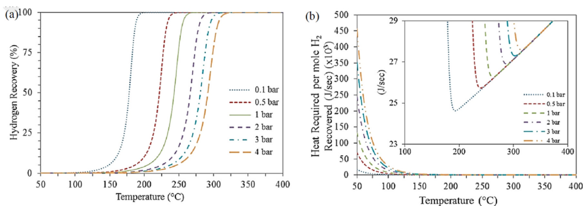
Fig. 7. (a) The equilibrium conversion of perhydridibenzyltoluene dehydrogenation at different pressures and temperatures. The results represent the maximum thermodynamically achievable hydrogen recovery under the given conditions, not the experimentally determined hydrogen recovery. (b) Heat energy required per second to release 1 mol of hydrogen during the dehydrogenation of perhydridibenzyltoluene over Pt/Al 2 O 3 catalyst [69].
