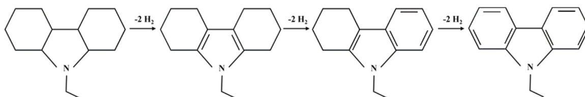
Fig. 6. Stepwise dehydrogenation mechanism of perhydro-N-ethylcarbazole (12H-NECZ) showing sequential hydrogen release via 8H- and 4H-NECZ intermediates [68].
