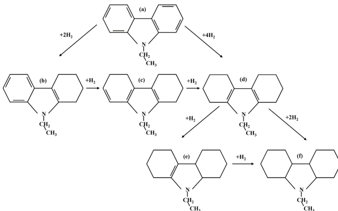
Fig. 4. Reaction pathway for the hydrogenation of N-ethylcarbazole (NEC) over Ru-based catalysts [62].
