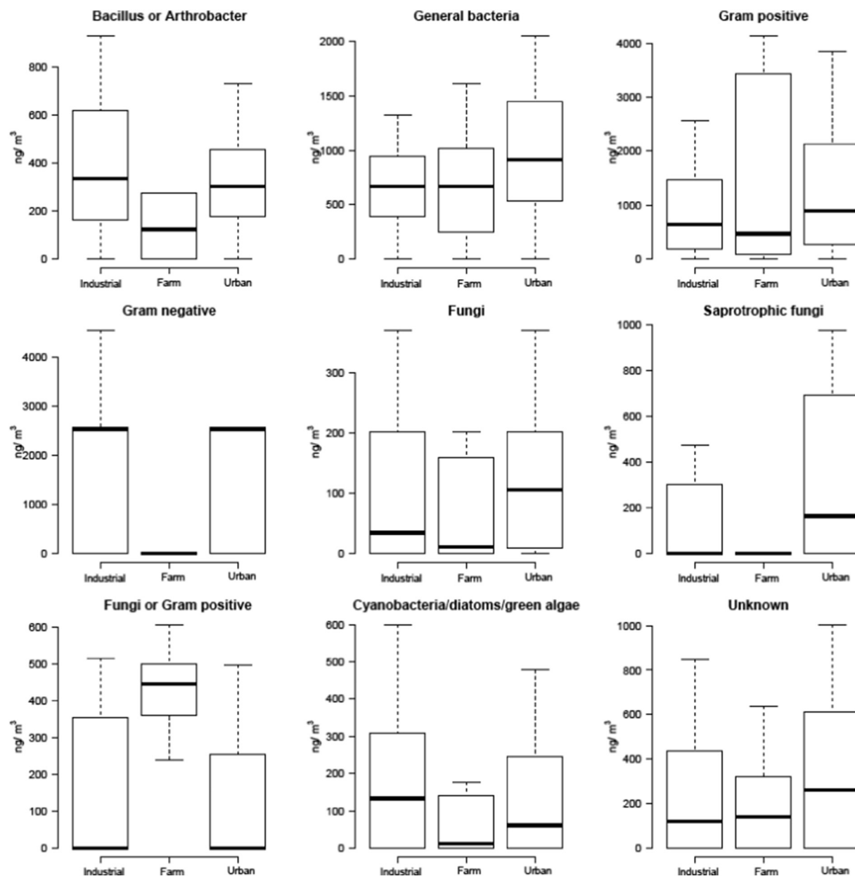
Fig. 5. Boxplot for grouped PLFAs concentrations expressed in \text{ng m}^{-3} in the three environments, namely industrial, farms and urban environments.
