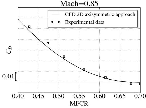
FIGURE 6: Comparison of nacelle drag as a function of massflow capture ratio for the 2D axisymmetric nacelle configuration
