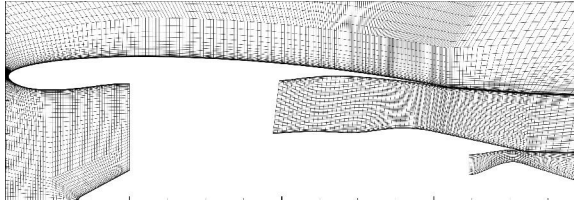
FIGURE 2: Computational mesh for the 2D axisymmetric numerical model
