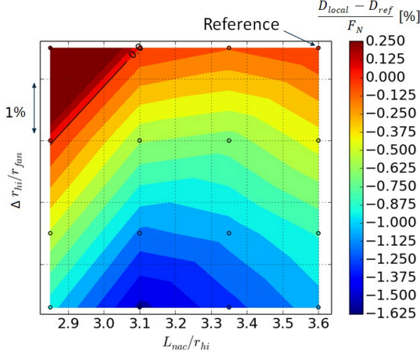
FIGURE 9: Mid-cruise normalised drag changes with net thrust ((D_{local} - D_{ref})/F_N) across the r_{hi}/r_{fan} - L_{nac}/r_{hi} design space considered. D_{ref} refers to the nacelle drag for the reference nacelle with L_{nac}/r_{hi} = 3.6 and \Delta r_{hi}/r_{fan} = 0\%
