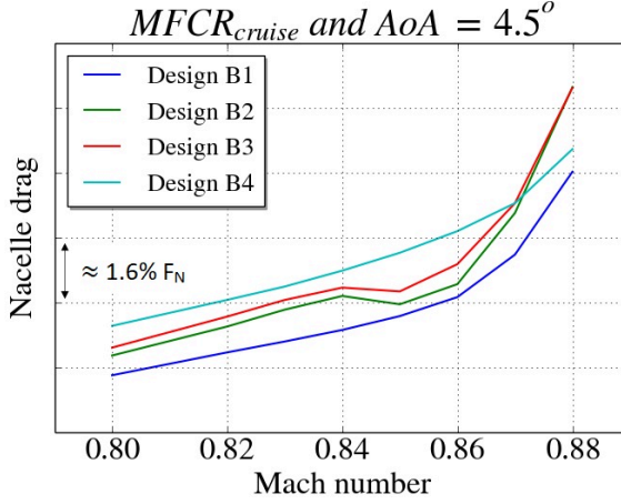
FIGURE 12: Comparison of nacelle drag as a function of Mach number for the downselected 3D nacelles
