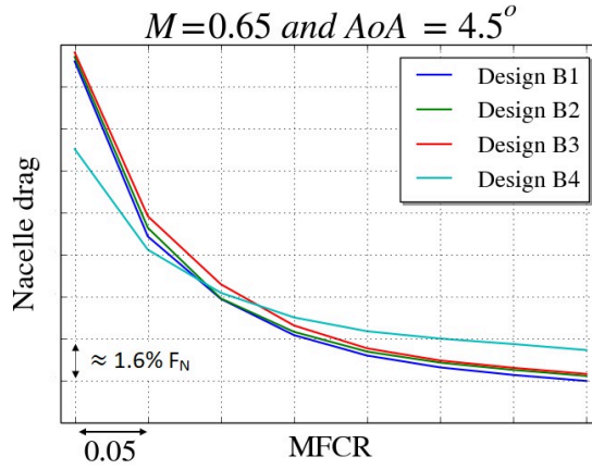
FIGURE 13: Comparison of nacelle drag as a function of massflow capture ratio for the downselected 3D nacelles
