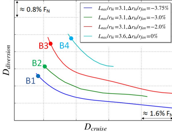
FIGURE 10: Projection into the D_{cruise} - D_{diversion} space of the Pareto fronts for the 3D configurations
