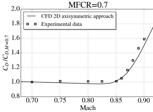
FIGURE 4: Comparison of nacelle drag as a function of Mach number for the 2D axisymmetric nacelle configuration
