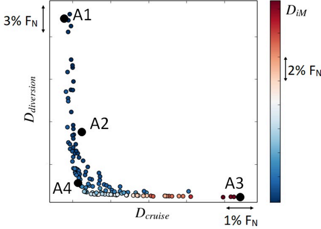
FIGURE 7: Pareto front for the reference 2D axisymmetric aero-engine nacelle with L_{nac}/r_{hi} = 3.6 and \Delta r_{hi}/r_{fan} = 0\%
