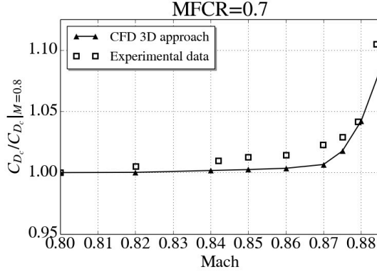
FIGURE 5: Comparison of nacelle drag as a function of Mach number for the 3D nacelle configuration
