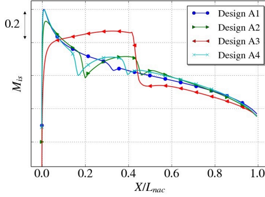
FIGURE 8: Isentropic Mach number distribution for downselected nacelles of the reference 2D axisymmetric MOO
