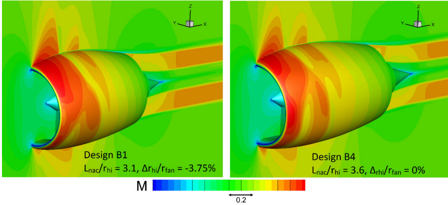
FIGURE 11: Mach number comparison for the downselected compact design B1 and the baseline architecture B4
