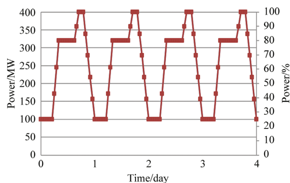
Figure 16 Total power produced during 4 days (winter).
