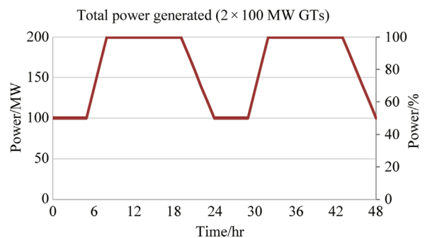
Figure 12 Total power produced by 2 \times 100 MW gas turbine (summer).
