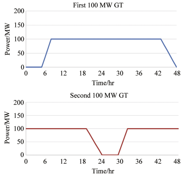
Figure 11 2 \times 100 MW gas turbine power plant Start–Stop operating scenario (summer).
