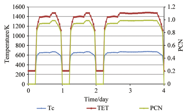
Figure 17 TET, Tc and PCN for GT-1 Start-Stop scenario (winter).
