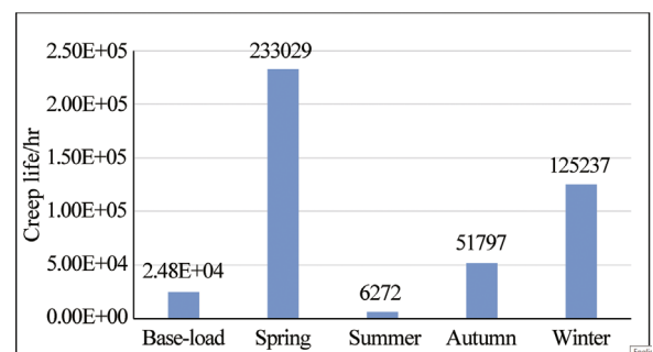
Figure 18 Creep life in 4 seasons for reference engine.
