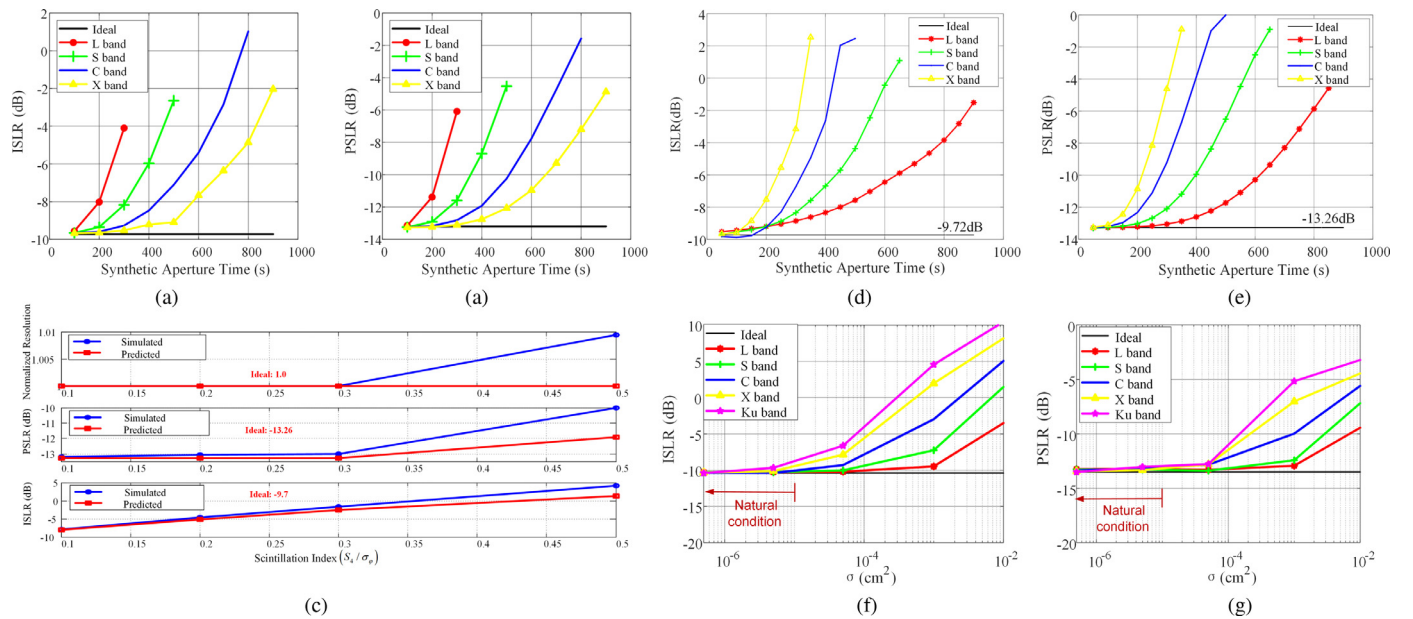
Fig. 3. Performances of GEO SAR azimuth focusing in the presence of atmospheric effects. 18° inclination GEO SAR above the equator (with a velocity of ~800 m/s) was adopted. (a) Integrated sidelobe ratio (ISLR) and (b) peak-to-sidelobe ratio (PSRL), as affected by the background ionosphere [50]. The fitting coefficients of TEC were q_1 = 6.8 \times 10^{-3} \text{TECU/s} , q_2 = 7.32 \times 10^{-6} \text{TECU/s}^2 , q_3 = 4.42 \times 10^{-12} \text{TECU/s}^2 . (c) Predicted and simulated performances in the L-band GEO SAR affected by ionospheric scintillation [54]. (d) ISLR and (e) PSRL, as affected by the background troposphere [67]. (f) ISLR and (g) PSRL affected by tropospheric turbulence, where \sigma is the refractive index variance [67]. An integration time of 120 s was set for (c). One can see from the simulation that the higher band GEO SAR works in, the weaker the ionospheric effects are, and the stronger the tropospheric effects are.
