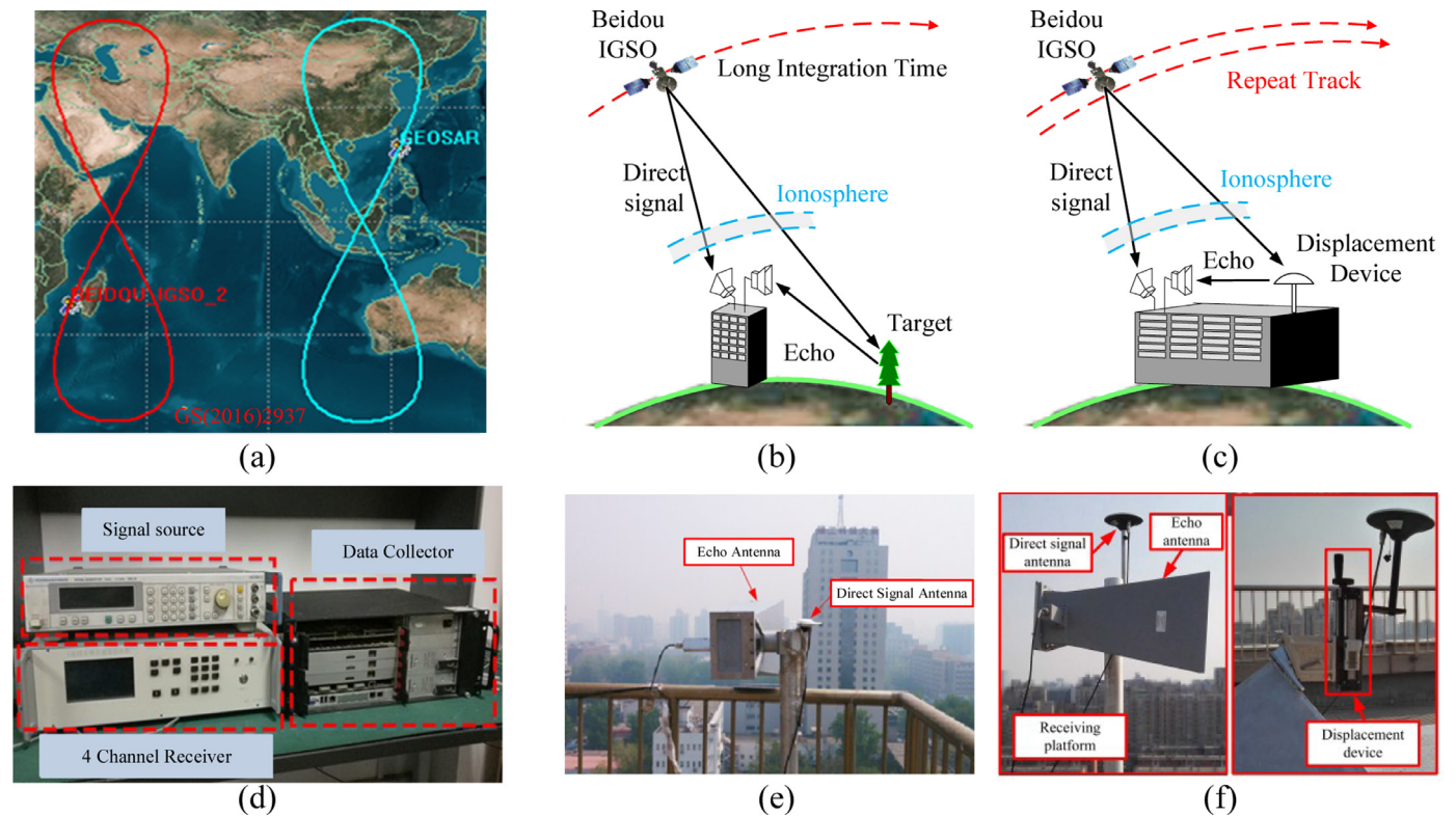
Fig. 6. GEO SAR equivalent verification experiment based on the Beidou IGSO satellite. (a) Nadir points of the inclined GEO SAR and Beidou IGSO satellites. (b) Geometry adopted for the SAR imaging experiment and TomoSAR experiment. (c) Geometry adopted for the 3D deformation retrieval experiment. (d) Data-collection equipment. (e) Antennas adopted for the SAR imaging experiment and TomoSAR experiment. (f) Antennas adopted for the 3D deformation retrieval experiment.
