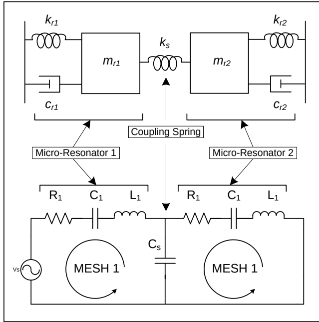
Figure 4: (Top) Lumped mechanical equivalent model of a 2nd order bandpass filter with mass-less coupling springs, (Bottom) corresponding electrical equivalent LCR network neglecting static capacitance at the I/O ports and utilizing an I-type coupling shunt capacitor
