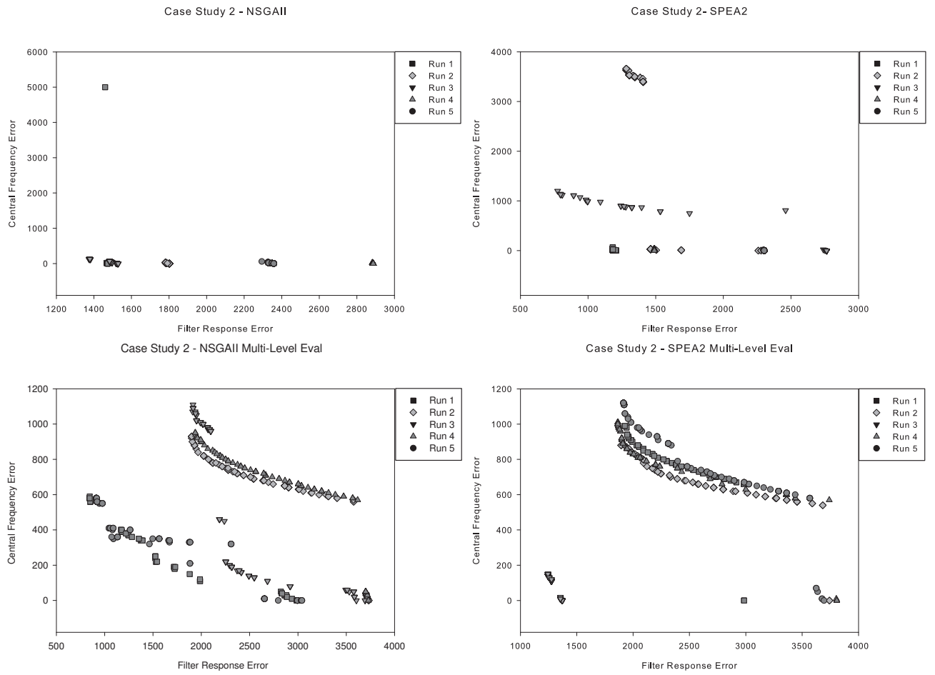
Figure 14: Case study 2 final population sets for both single and multi-level NSGAII and SPEA2
