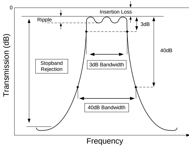
Figure 2: Bandpass filter parameter specifications [33]
