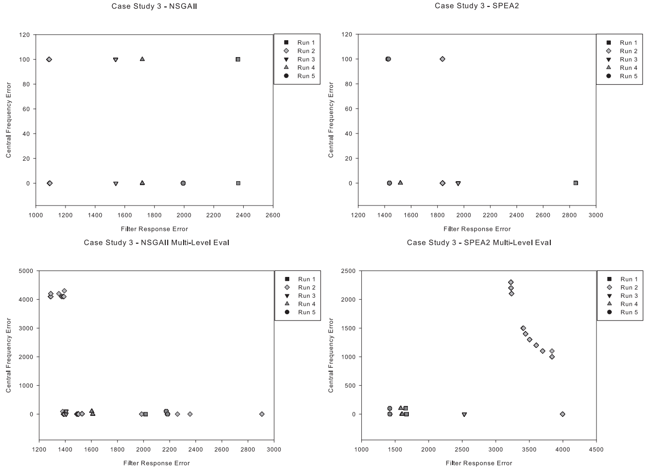
Figure 15: Case study 3 final population sets for both single and multi-level NSGAI and SPEA2
