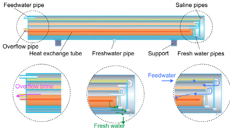
(b) Flow of feedwater and fresh water inside TSS
