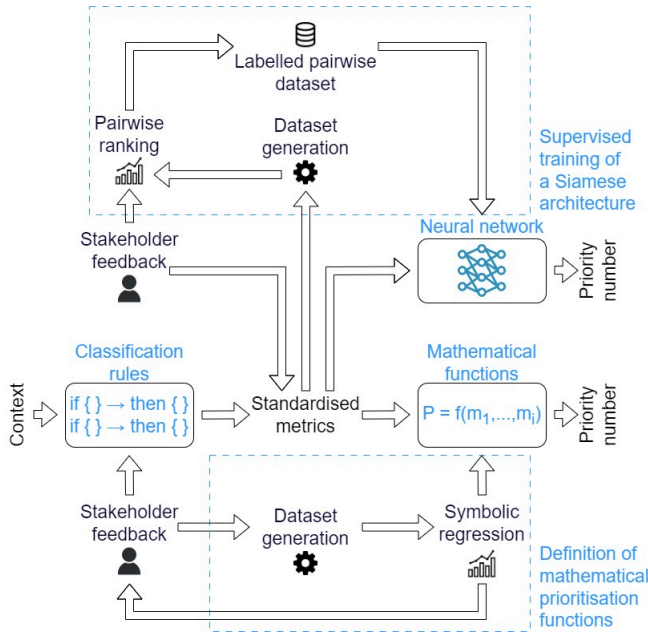
Fig. 4. Overview of the algorithmic solutions used for a preliminary study of dynamic non-binary prioritisation for UTM.
