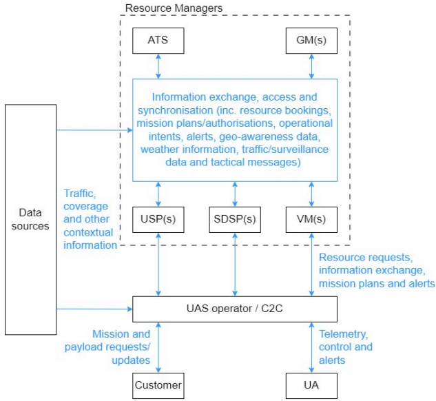
Fig. 1. Typical actors (black) and data flows (blue) in a UTM architecture.
