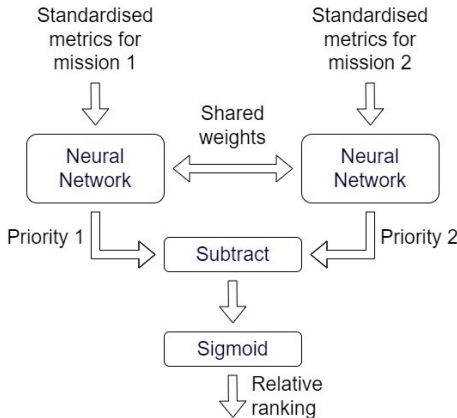
Fig. 5. Architecture of a Siamese network used to learn absolute priority mappings from pairwise expert decisions.
