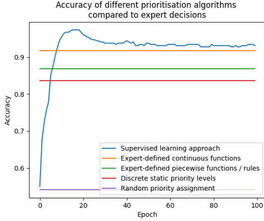
Fig. 12. Comparison of the accuracy of different priority computation techniques for simple use cases, when compared to expert decisions.
