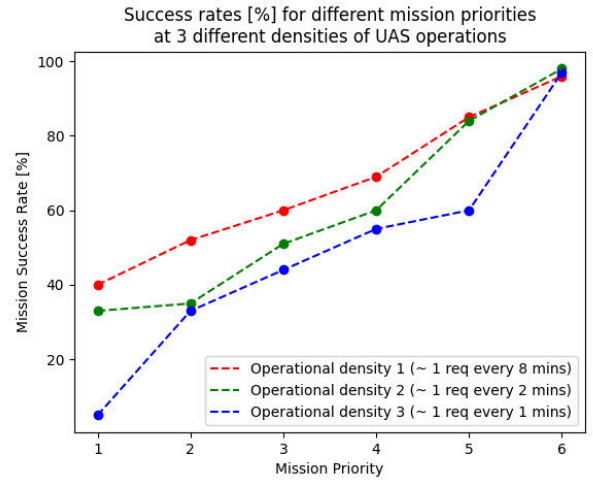
Fig. 6. Data-driven results showing the performance of a priority-driven resource allocation mechanism in a federated UTM ecosystem, for increasingly high operational densities (red to blue).
