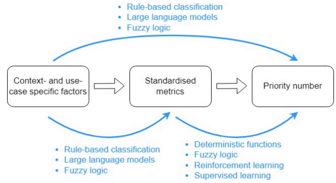
Fig. 3. Algorithms for context-to-priority mapping.
