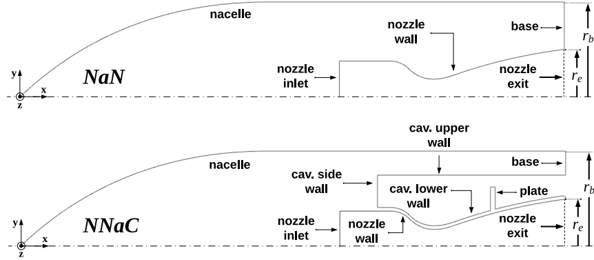
Fig. 1: Configurations under investigation: Nozzle and nacelle (top), Nozzle, nacelle and cavity (bottom)
