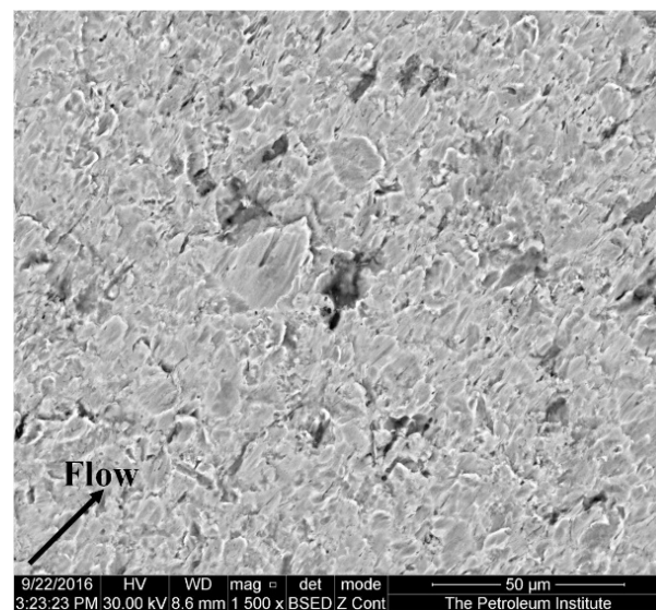
Figure 12. Surface of the specimen 2 mm away from the center after pure erosion test at 20 m/s and 600 mg/L.
