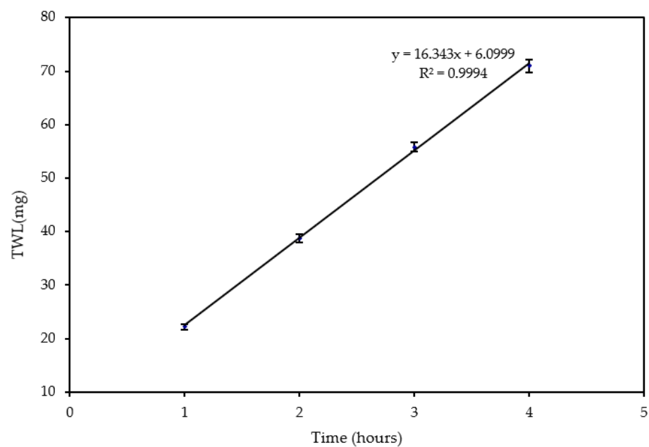
Figure 4. Change of TWL with respect to time at 20 m/s and 600 mg/L.
