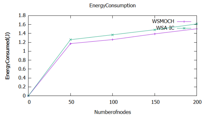
Fig 5.4: Energy consumption vs Number of Nodes
