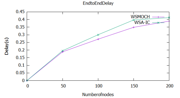
Fig.5.2 End-to-End Delay vs Number of nodes
