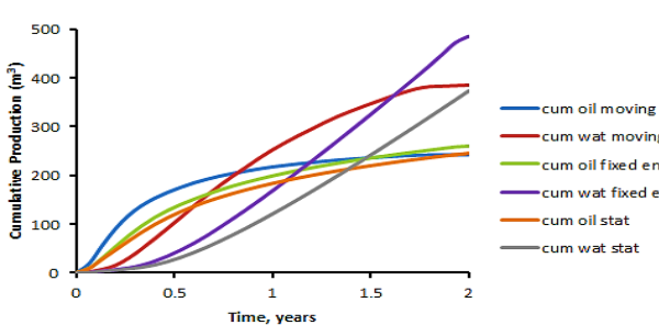
Figure 8: Total Production for the Three Optimization Cases
