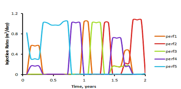
Figure 5: Injection Rates for Fixed-End RH
