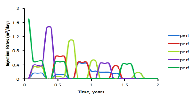
Figure 4: Injection Rates for Moving-End RH
