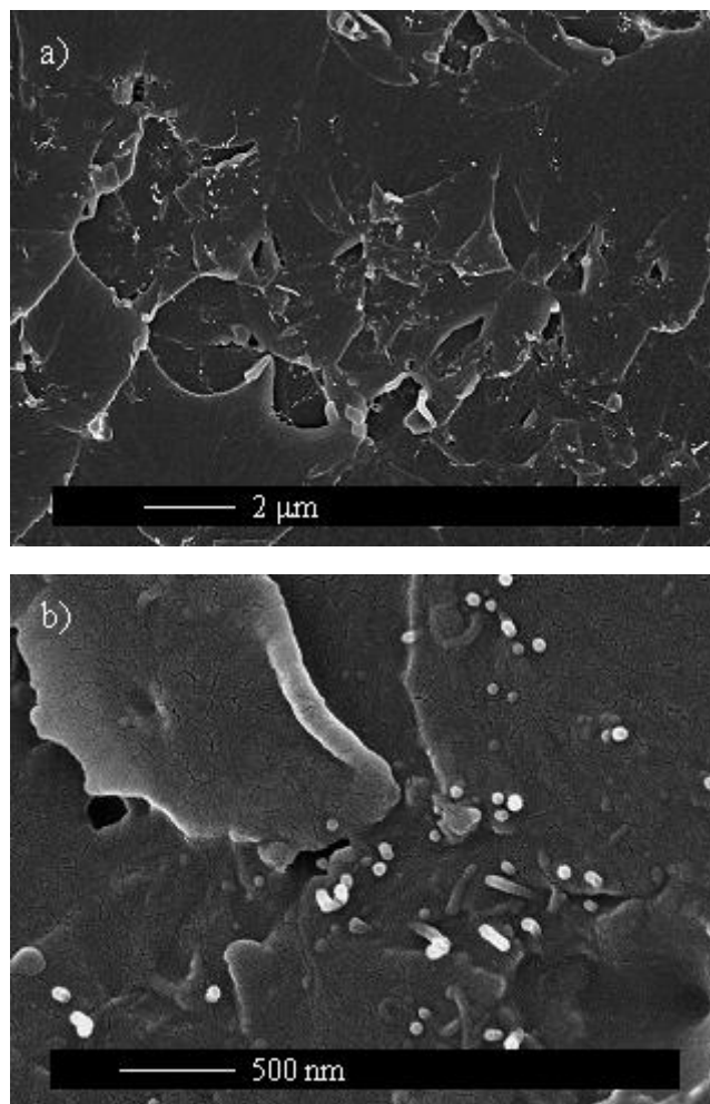
Fig. 6. Scanning electron micrographs (FEG-SEM) of cryo-fracture surfaces for (a) CN and (b) etched CRN.
