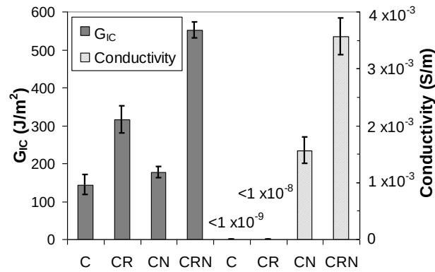
Fig. 8. Fracture energy, G_{IC} , and electrical conductivity of the formulations employed.
