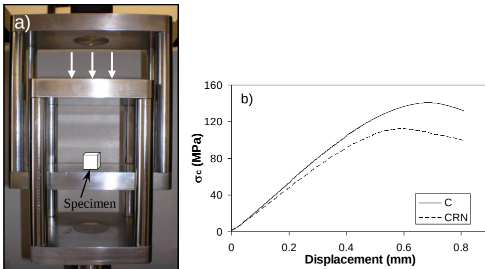
Fig. 4. (a) Compression cage, with a schematic of specimen loading (not to scale) (b) Stress- displacement curves under compression loading, for C and CRN samples.
