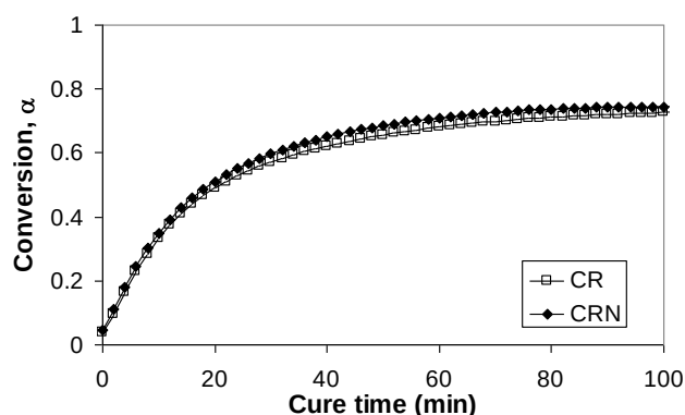
Fig. 3. Conversion versus cure time at 120°C, in the first 100 minutes. Conversion was determined by differential scanning calorimetry experiments, giving total reaction enthalpies as 449 and 380 J/g for CR and CRN formulations respectively. Conversion was determined using a horizontal integration baseline, method described fully in [6].
