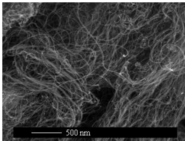
Fig. 2. Scanning electron micrograph (FEG-SEM) of NC-7000 multi-walled carbon nanotubes, as supplied, showing a highly-entangled structure.
