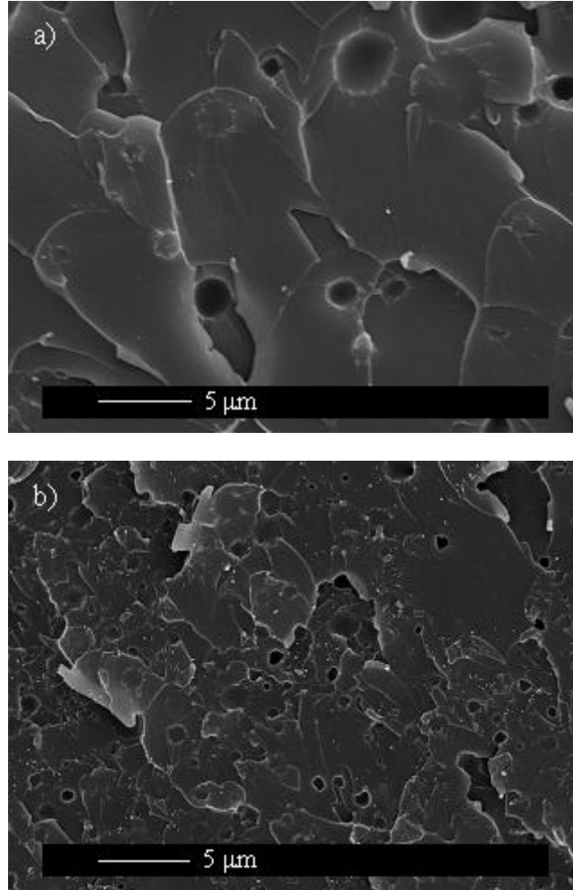
Fig. 7. Scanning electron micrographs (FEG-SEM) of etched fracture surfaces for (a) CR and (b) CRN.
