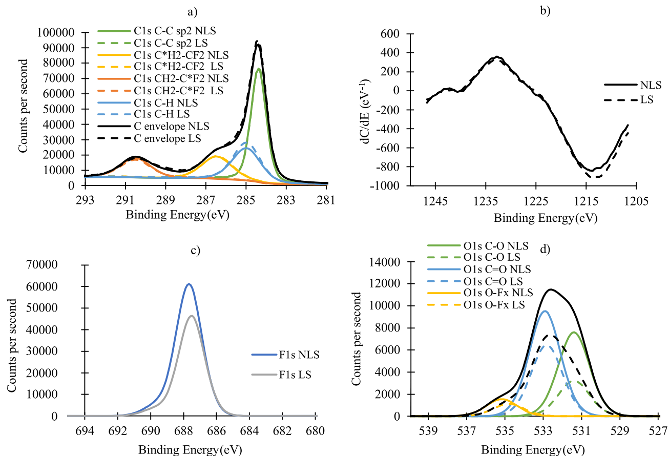
Fig. 18. Comparison of XPS results obtained for non laser-scribed (NLS) and for laser-scribed (LS) electrodes (K-bar set) with a pulse energy of 314 \mu J and a spacing of 100 \mu m: (a) C1s peaks, (b) Differentiated CKL1 peaks (Auger). The D parameter is 18.9 for NLS and 19.4 for LS, (c) F1s peaks and (d) O1s peaks. The C/O ratio was found to be 21.8 for NLS and 19.9 for LS.
