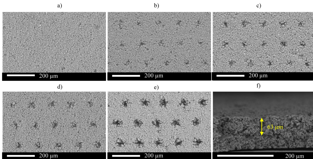
Fig. 6. K-bar set: micrographs taken at a 710x magnification of (a) non laser-scribed electrode and electrodes laser-scribed with a 140 \mu\text{m} spacing and 257 \mu\text{J} , 314 \mu\text{J} , 371 \mu\text{J} and 571 \mu\text{J} (b, c, d and e, respectively); (f) Cross-sectional micrograph (1433x) demonstrating the depth of holes in laser-scribed electrode identical to the one shown in (e).
