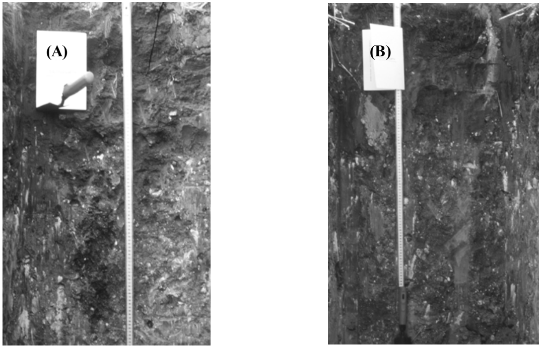
Fig. 3. Soil profile pits in Far Sweetbrier showing (A) and (B) Hanslope soil series.
