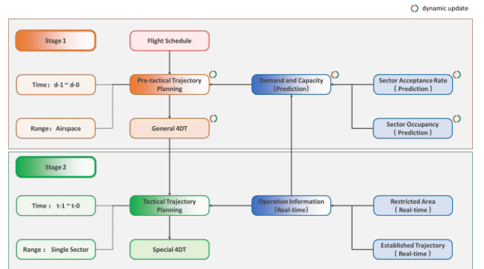
Figure 1. The pre-tactical-and-tactical integrated 4DT planning framework.
