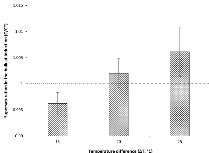
Fig. 3. Extent of supersaturation achieved in bulk solution at induction for the bulk crystal phase. For each \Delta T , saturation approaches a C/C^* \sim 1 (dashed line). The average and error bars for each \Delta T represent saturation data from each Re for that temperature difference and were repeated in triplicate ( n = 21 ). Experimental conditions: \Delta T 15–25 °C, Re 1300–2050, feed temperature 60 °C.
