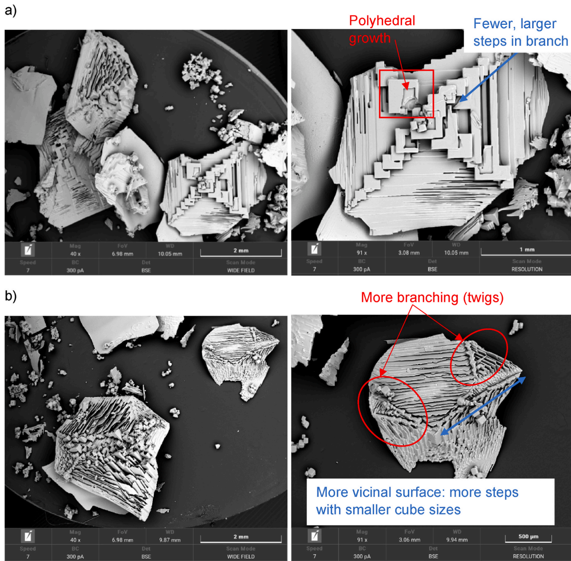
Fig. 7. High-resolution scanning electron microscopy (SEM) images of scaling formed at the membrane: (a) Re 1300; and (b) Re 2050. Experimental conditions: \Delta T 25 ^{\circ} C, feed temperature 60 ^{\circ} C.
