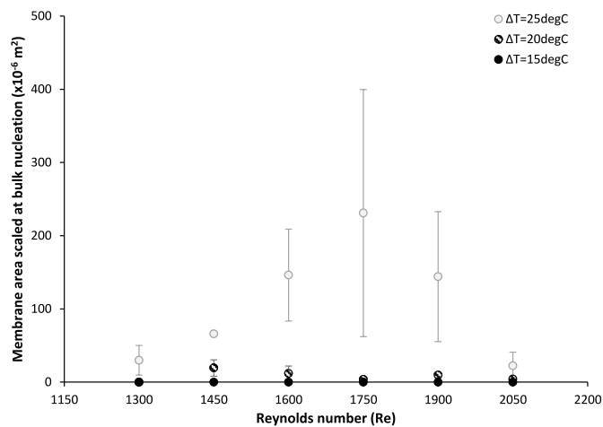
Fig. 8. Extent of scaling at the onset of bulk nucleation as determined by non-invasive digital microscopy. Experimental conditions: \Delta T 15–25 ^{\circ} C, Re 1300–2050, feed temperature 60 ^{\circ} C. Data repeated in triplicate.
