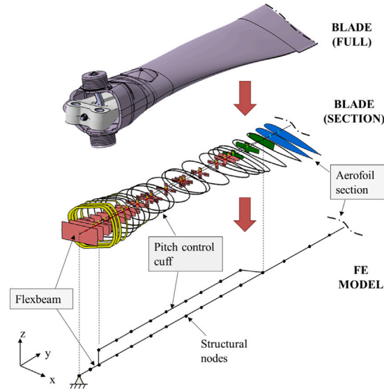
Fig. 2. Schematic of the FE modelling principle.
